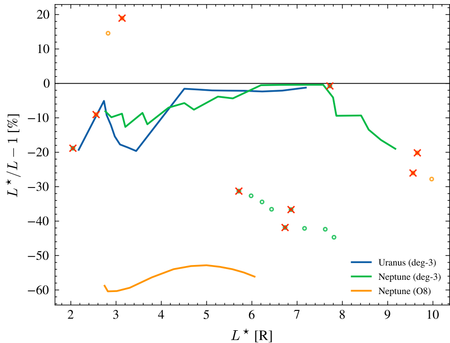
(b) dipole-L failure; x: fold points ( J=0 )
