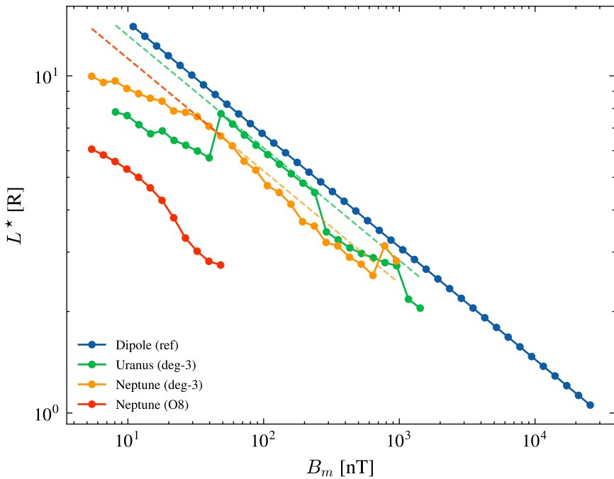
(a) L^\star(B_m) tables; dashed: dipole reference L
