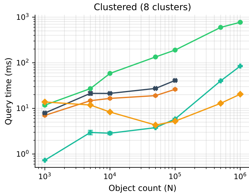
Query Time vs. Object Count (512 queries, mean \pm std, 3 runs)
