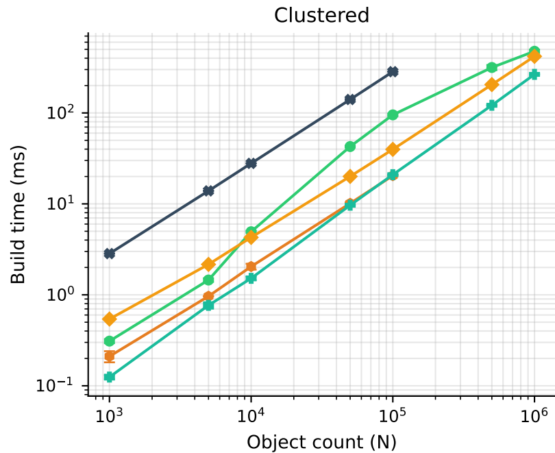
Build Time vs. Object Count (mean \pm std, 3 runs)
