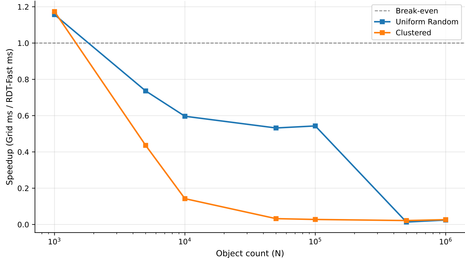
RDТ-Fast Query Speedup vs. Uniform Grid > 1.0 = RDТ-Fast is faster
