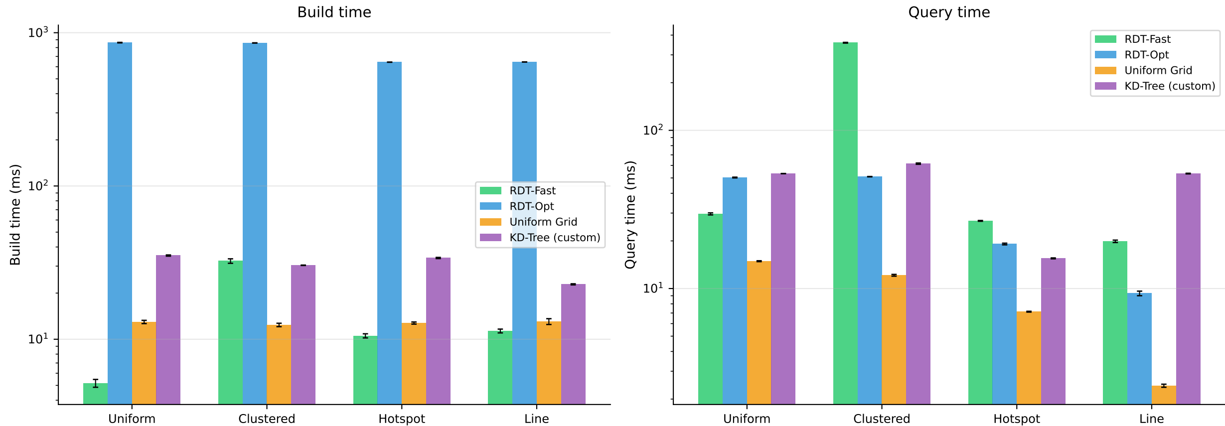
Build & Query Time at N=50,000 (mean \pm std, 3 runs)
