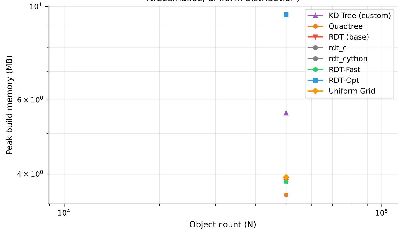
Peak Memory During Build (tracemalloc, uniform distribution)
