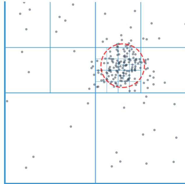
Quadtree 4-way split at threshold
