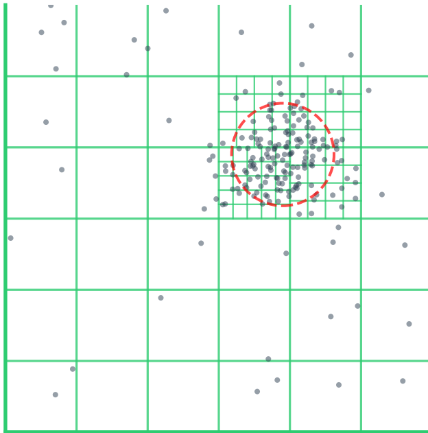
RDT g(n) = \text{floor}(\log(n+1)^\alpha)
