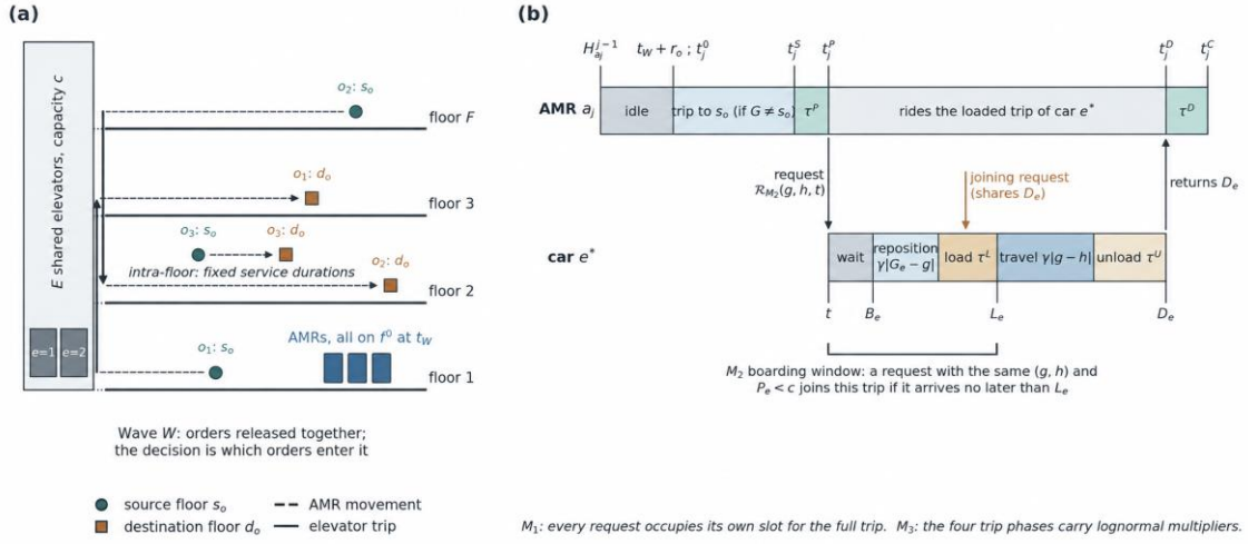
Fig. 1. Problem setting and serial reservation of one order. (a) A multi-story warehouse in which an AMR fleet shares E elevators. A wave is a set of orders with source and destination floors; AMRs change floors only by elevator trips, and all resources start on a common floor f^0 at the release epoch t_w . (b) Reservation of one order under the true co-occupancy batching evaluator M_2 (Section 3.5.1). The panel shows the clock of the assigned AMR (availability, readiness, start, pickup, and delivery), the waiting time, and the four phases of the loaded elevator trip (repositioning, loading, travel, and unloading). A request with the same origin and destination floors can join the trip while capacity remains, until loading ends at L_e . Durations are illustrative.
