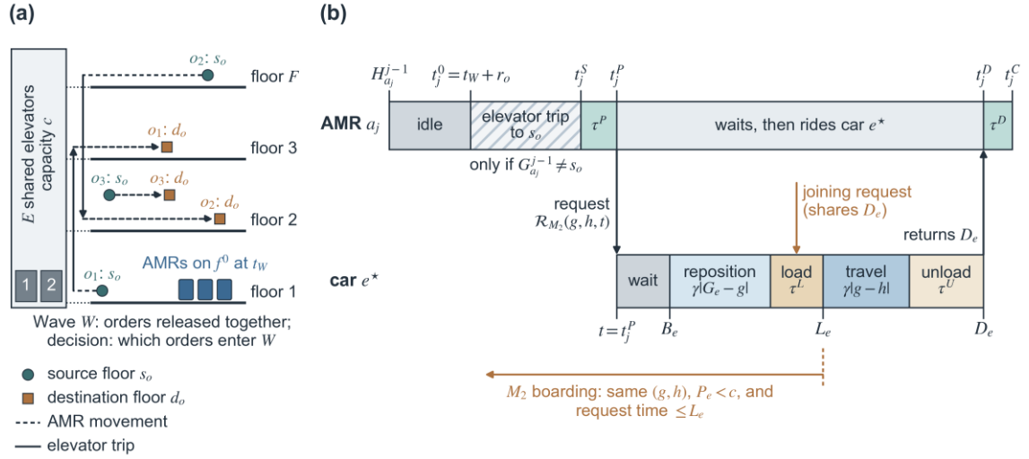
Fig. 3.1. Problem setting and serial reservation of one order. (a) A multi-story warehouse in which an AMR fleet shares E elevators. The decision is which n orders from the order pool form the wave W released at t_w . For each order, an AMR carries a load from its source floor to its destination floor. AMRs change floors only by elevator trips, and a car carries up to c AMRs traveling between the same pair of floors. All AMRs and cars start on a common floor f^0 , drawn as floor 1.
