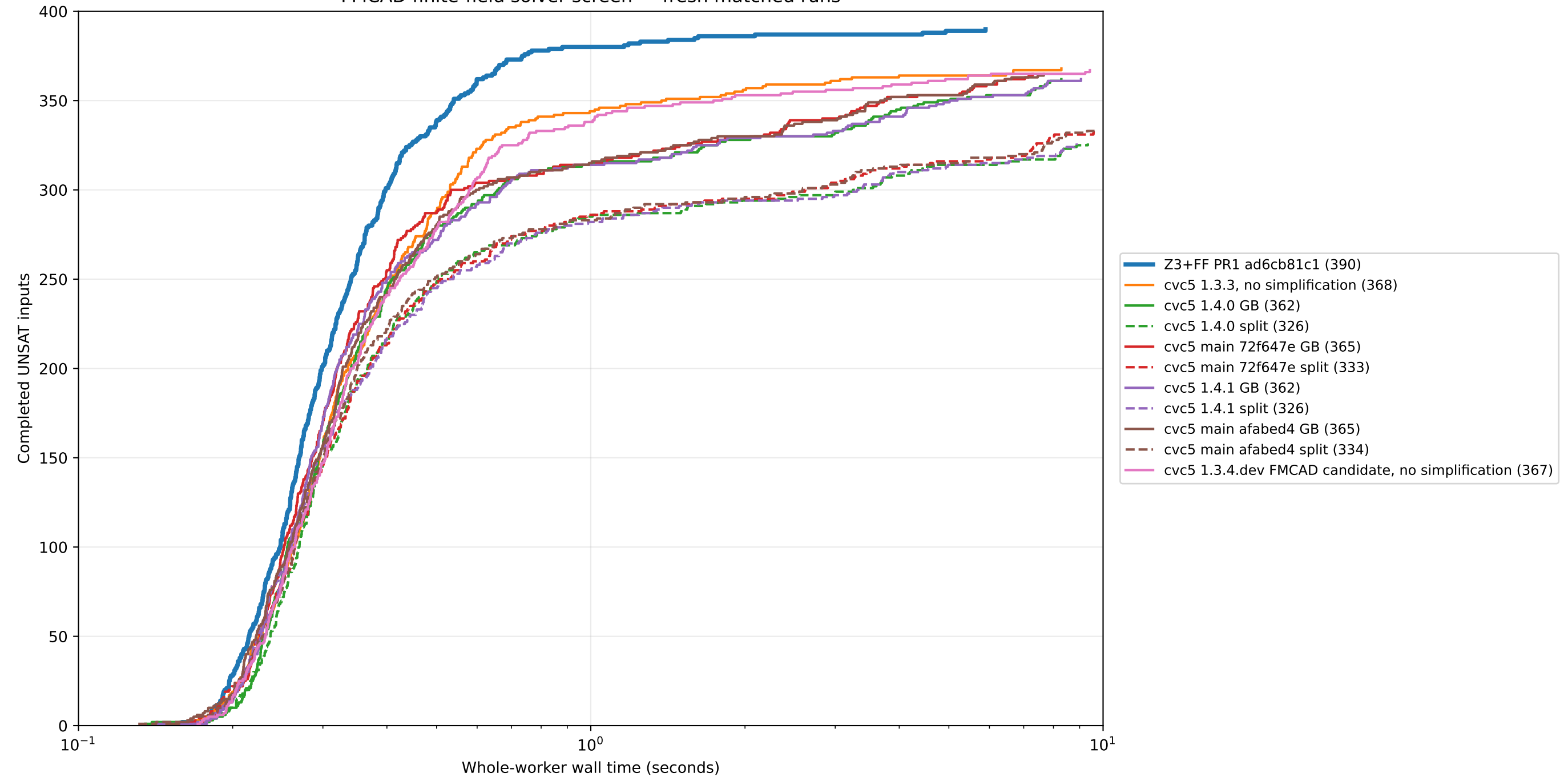
FMCAD finite-field solver screen — fresh matched runs
