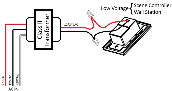
Figure 1. Wiring
