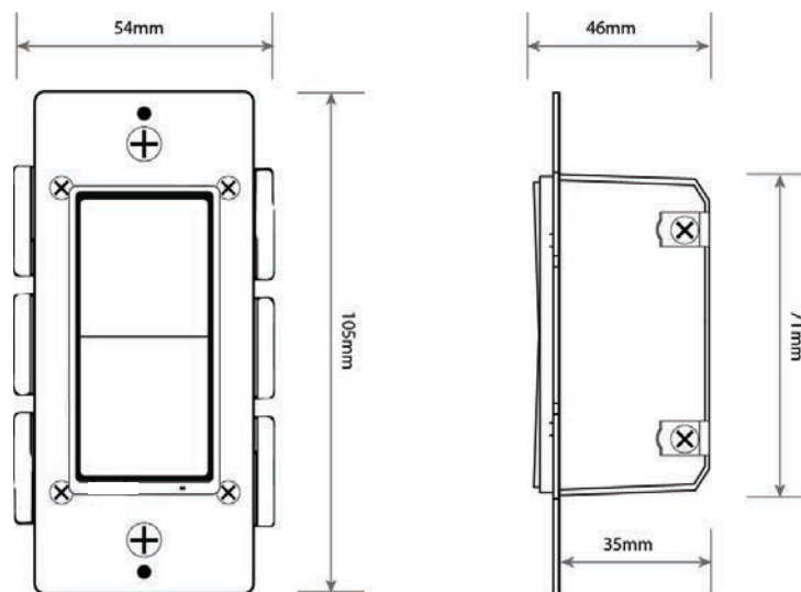
Figure 1. In-Wall Switch Dimensions
