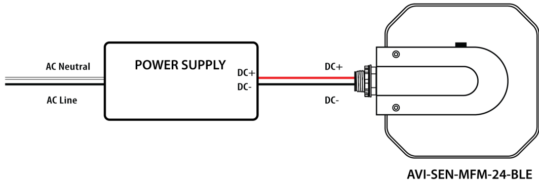
Figure 3. Wiring Diagram
