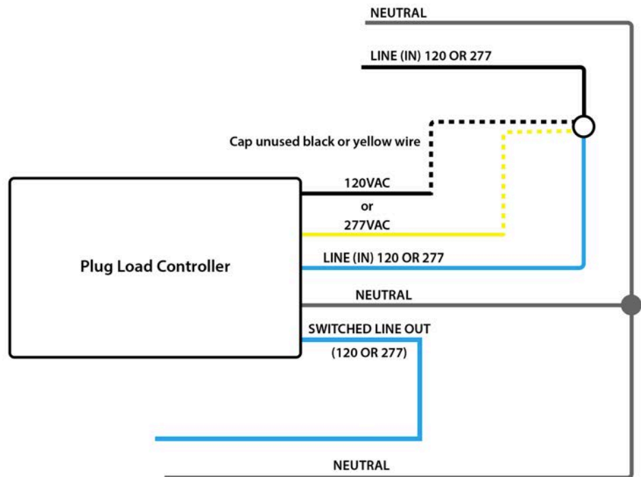
Figure 2. Wiring Diagram
