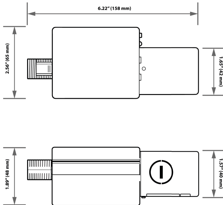
Figure 1. Dimensions
