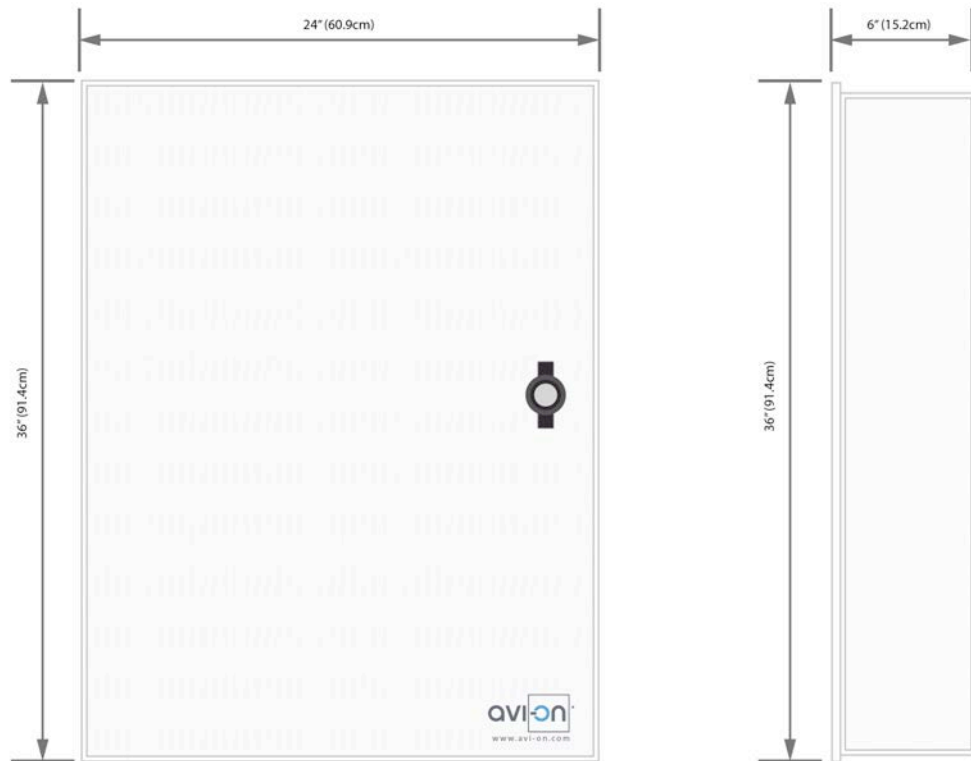
Assembly Dimensions
