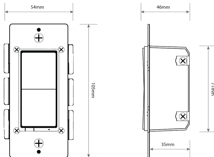
Figure 1. In-Wall Dimmer Dimensions
