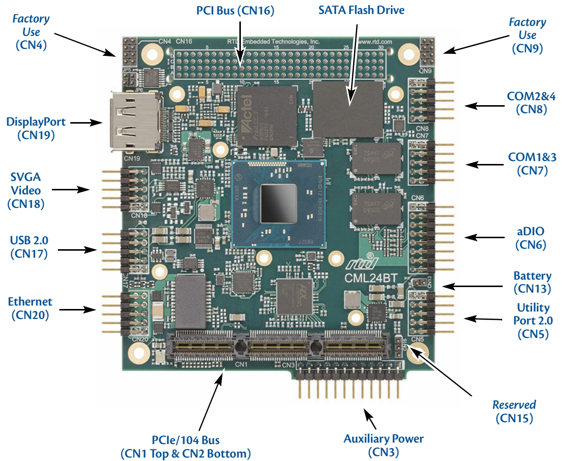
Figure 5 CML24BT cpuModule (top view)
