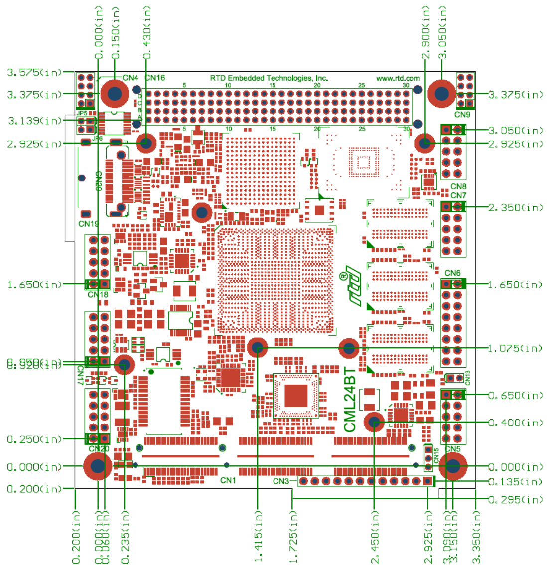
Figure 8 CML24BT Physical Dimensions ( \pm 0.005 inches)
