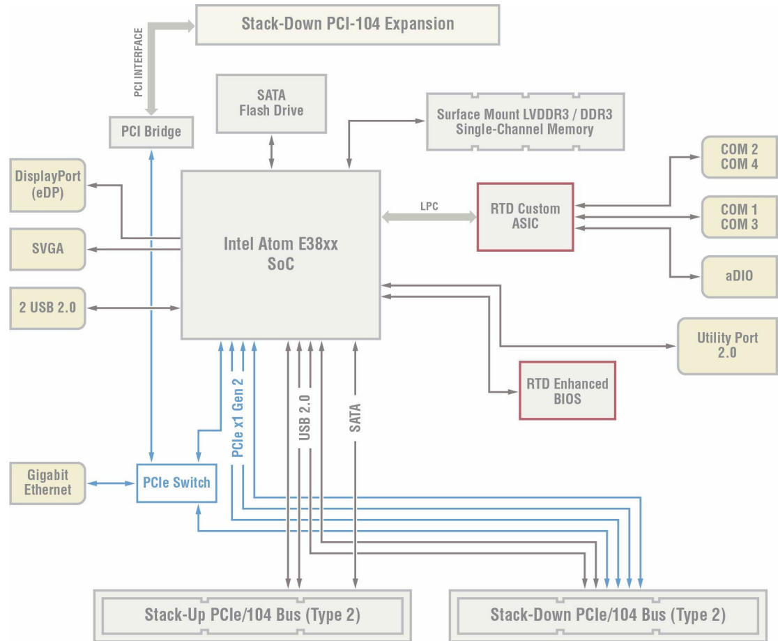
Figure 2 CML24BT cpuModule Simplified Block Diagram
