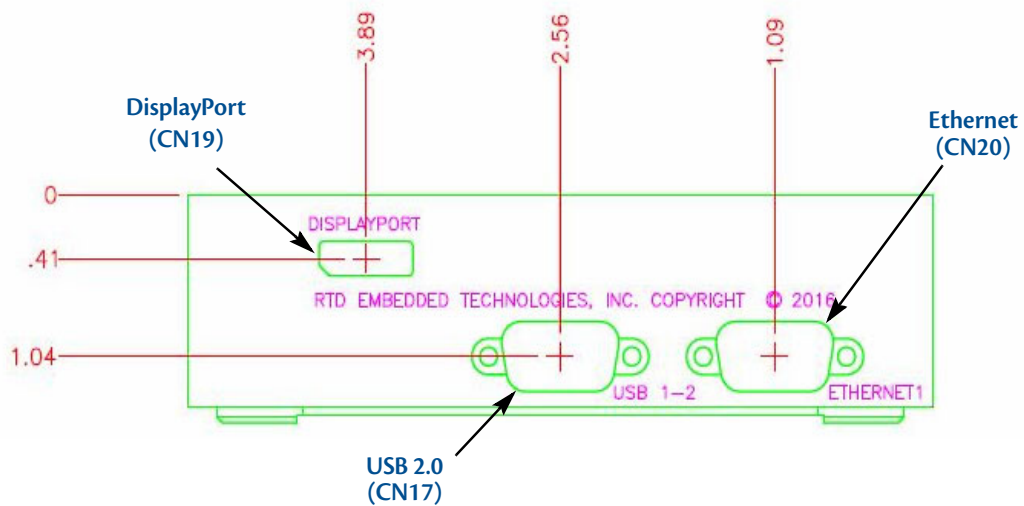
Figure 17 IDAN-CML24BT Back Panel
