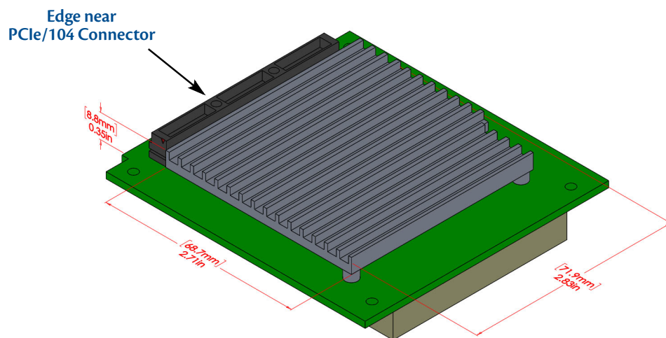
Figure 10 CML24BTD1330 Heatsink
