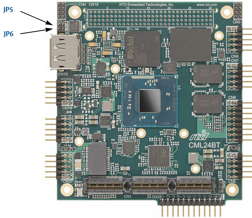
Figure 7 CML24BT Jumper Locations (top side)
