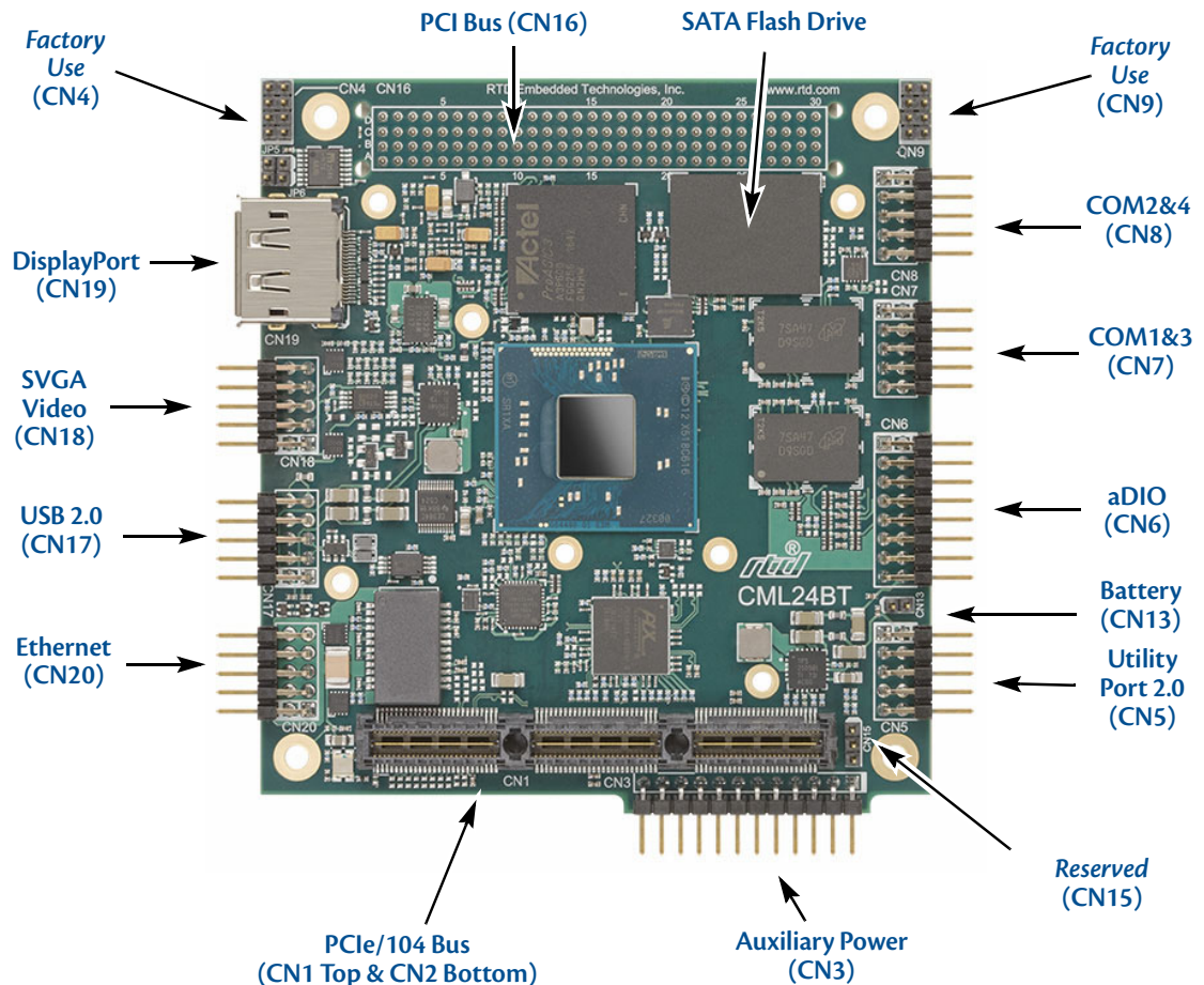
Figure 1 CML24BT cpuModule (top view)
