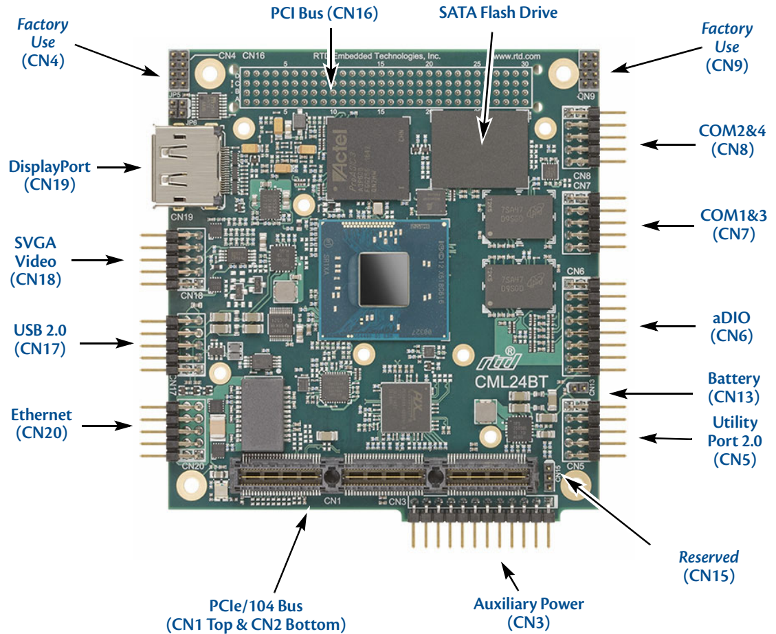
Figure 3 CML24BT Connector Locations
