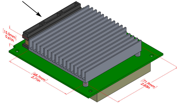
Figure 11 CML24BTQ1910 Heatsink
