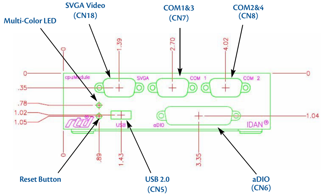
Figure 16 IDAN-CML24BT Front Panel
