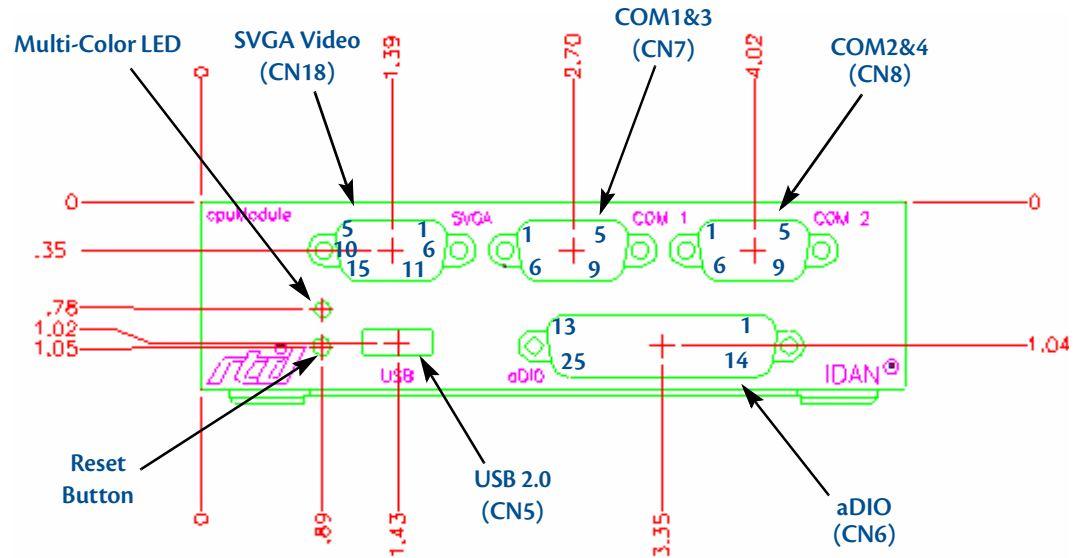
Figure 15 IDAN-CMX34BT Front Panel
