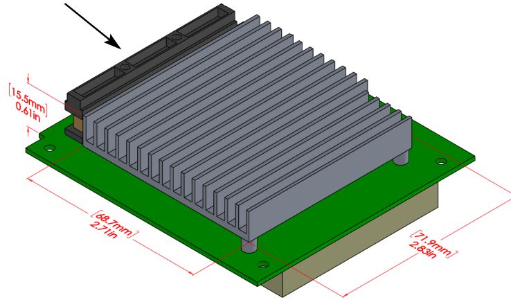
Figure 11 CMX34BTQ1910 Heatsink
