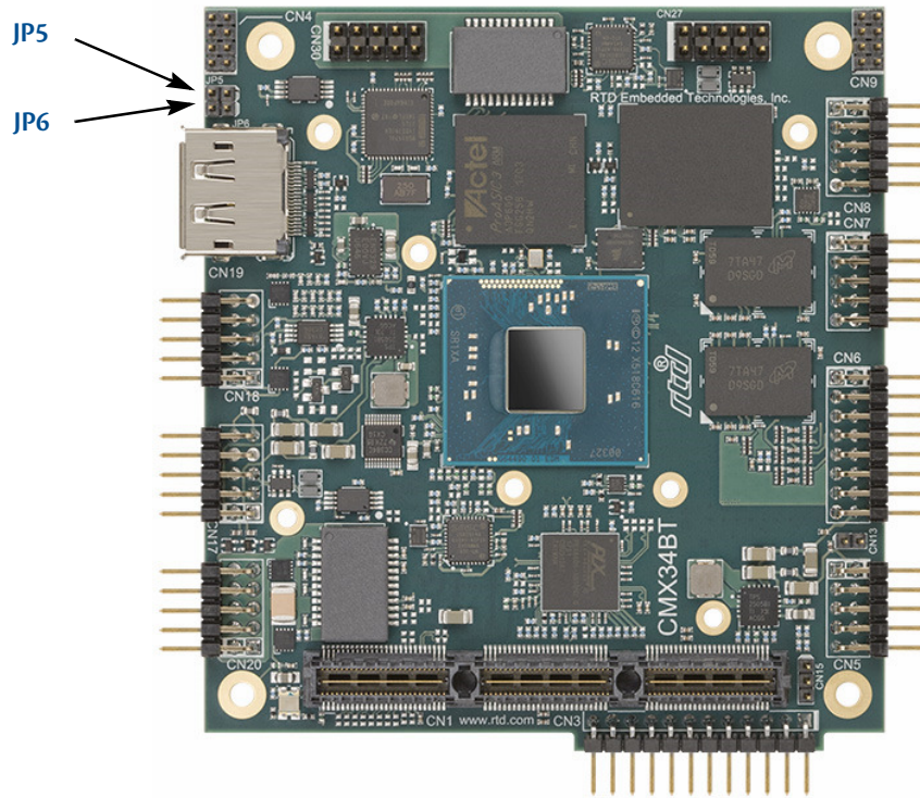
Figure 7 CMX34BT Jumper Locations (top side)
