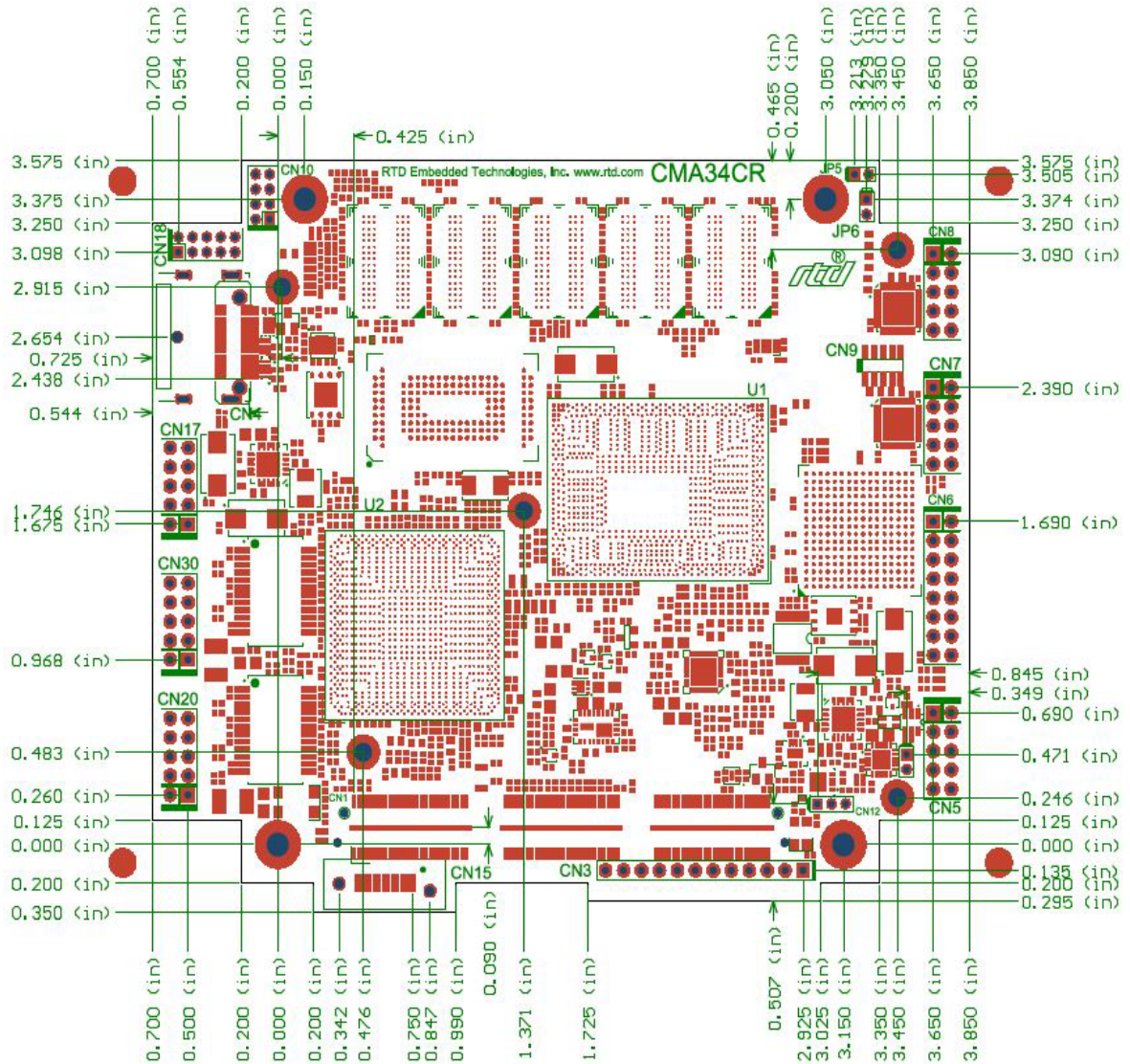
Figure 8 CMA34CR Physical Dimensions ( \pm 0.005 inches)
