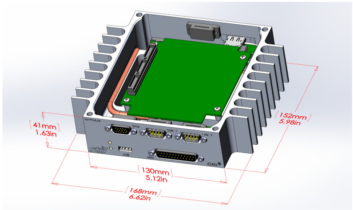
Figure 11 IDAN-CMA34CR Frame Dimensions
