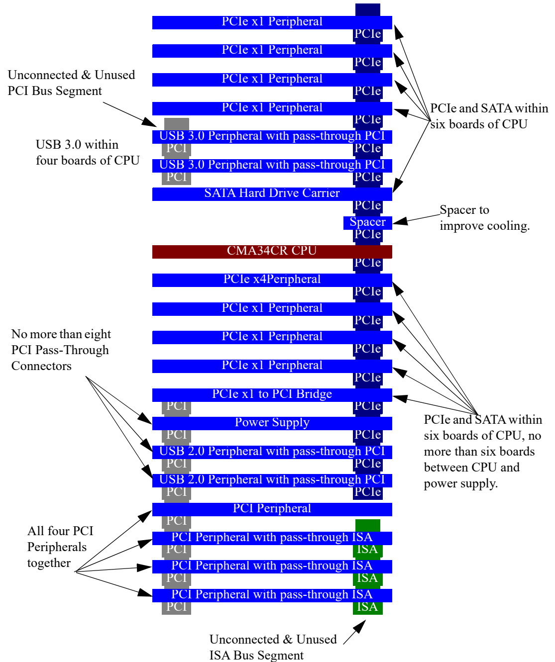
Figure 4 System Stacking Example
