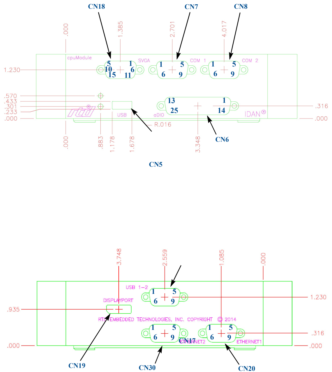
Figure 10 IDAN-CMA34CR Connector Pin Orientation
