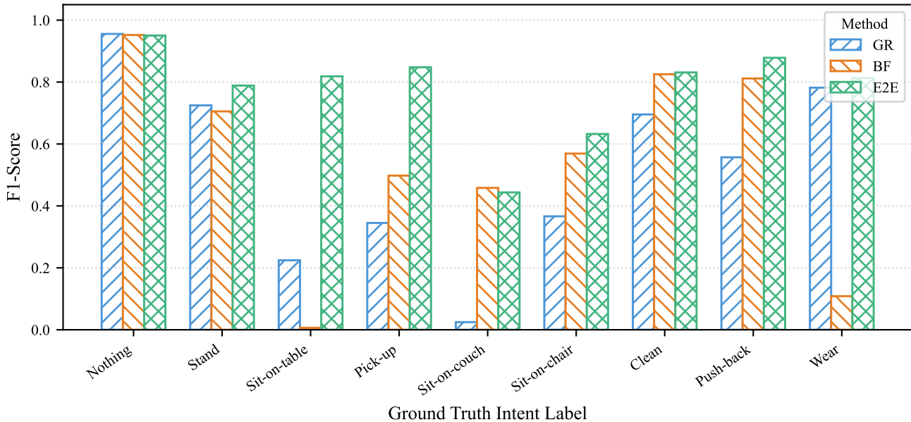
Per-Class F1-Score Across Three Methods (sub6)
