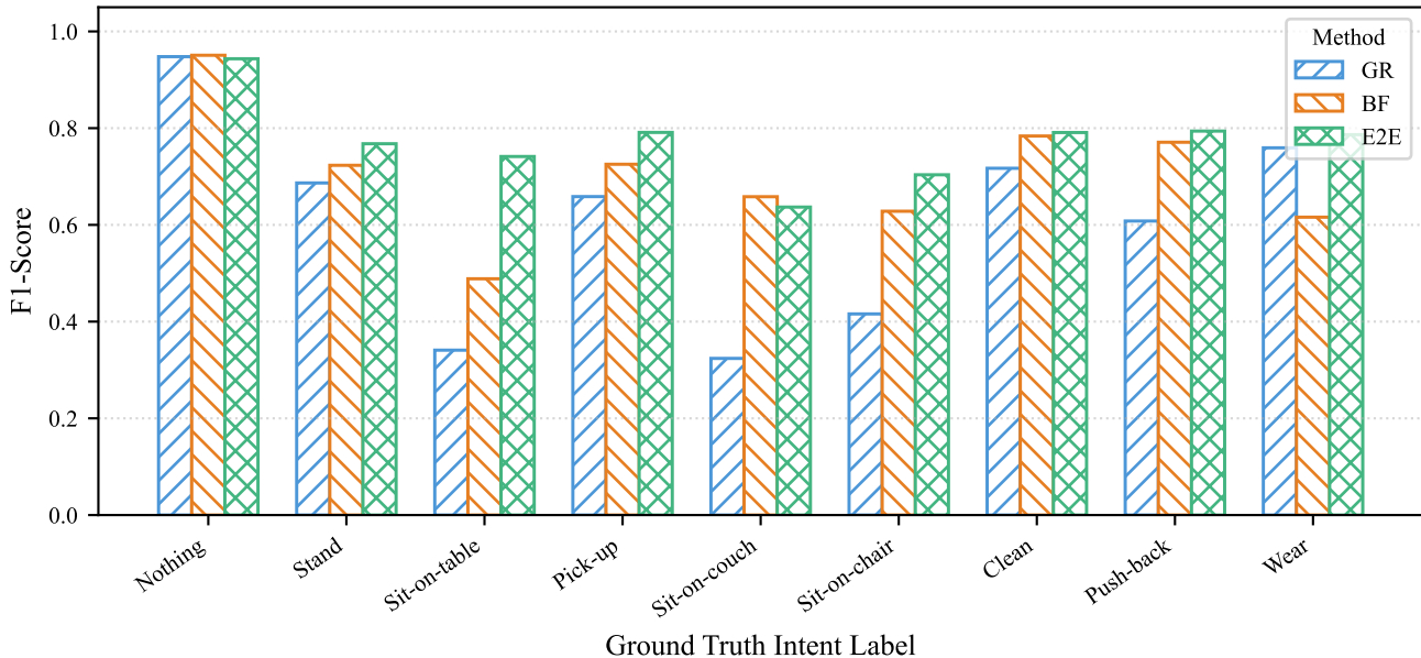
Per-Class F1-Score Across Three Methods
