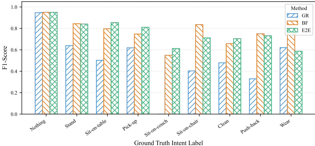
Per-Class F1-Score Across Three Methods (sub3)
