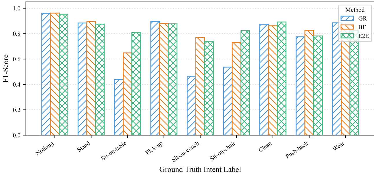
Per-Class F1-Score Across Three Methods (sub4)
