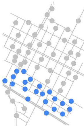
Feature set
