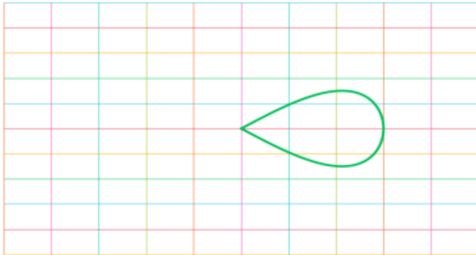
Figure 3.1 — Holographic Ledger: Boundary Pattern
