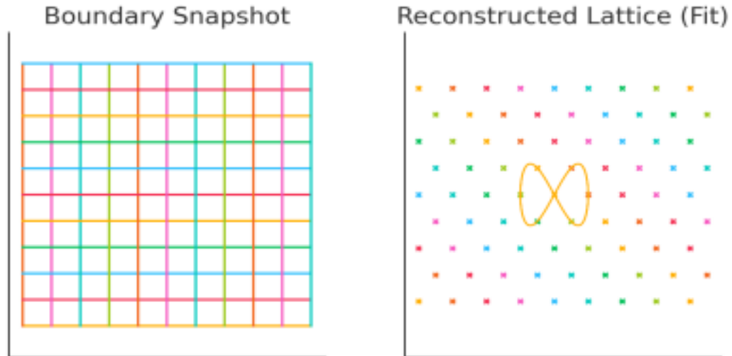
Figure 11.2 — Holographic Consistency
