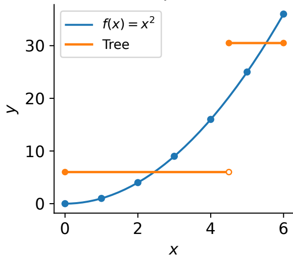
Depth 1
