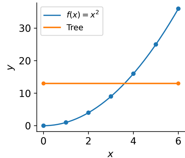
Root leaf
