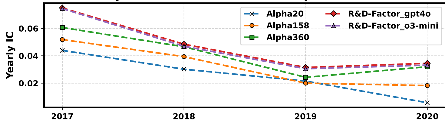
(a) Yearly IC: R&D-Factor (based on Alpha 20) vs Baseline
