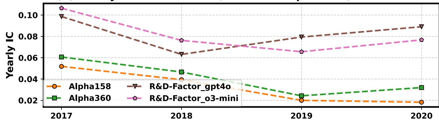
(b) Yearly IC: R&D-Factor (based on Alpha 158) vs Baseline
