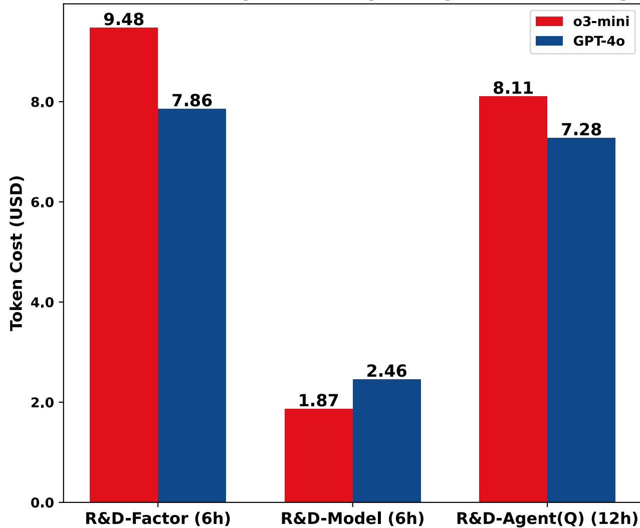
Total Token Expenditure per Experiment Group
