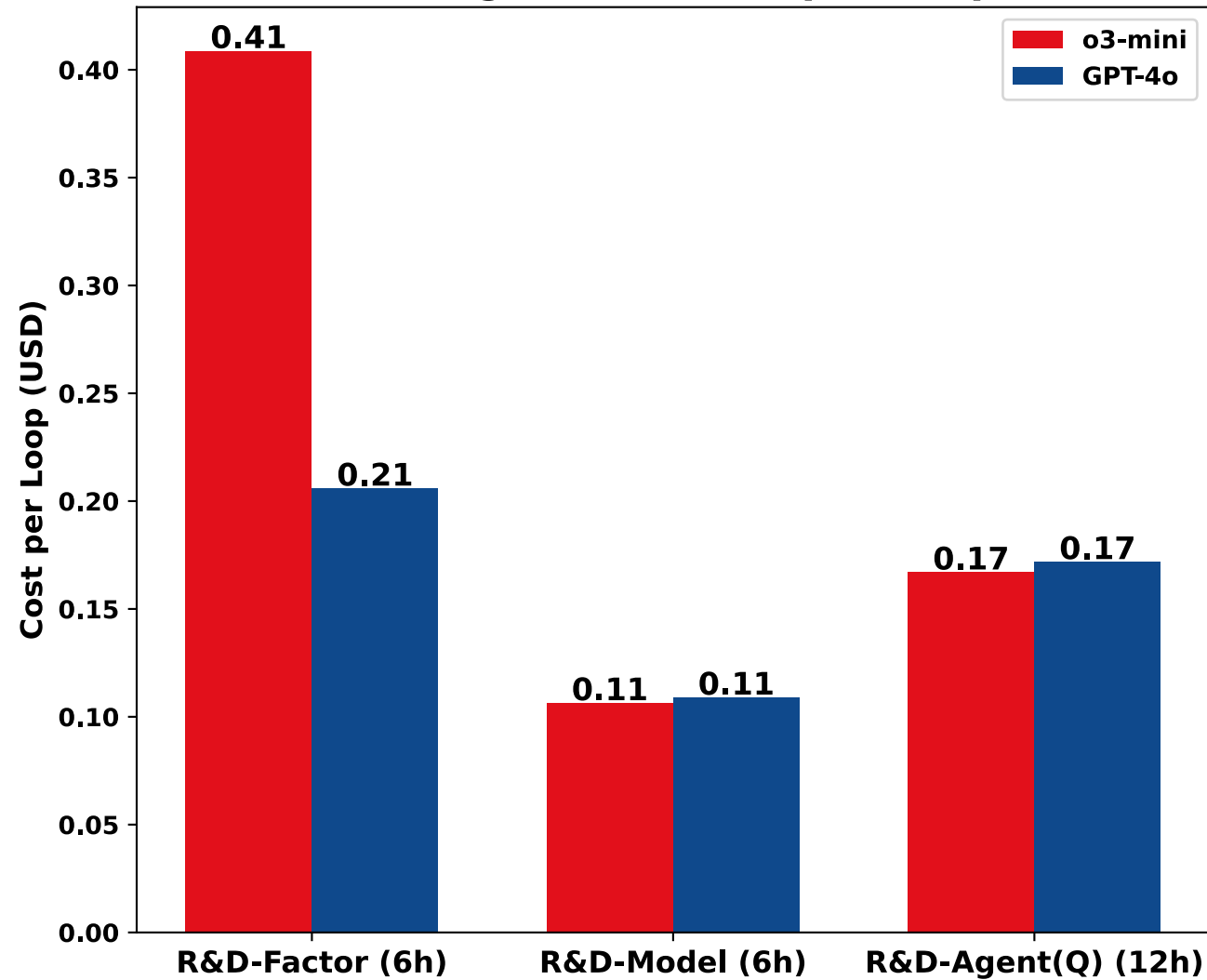
Average Token Cost per Loop
