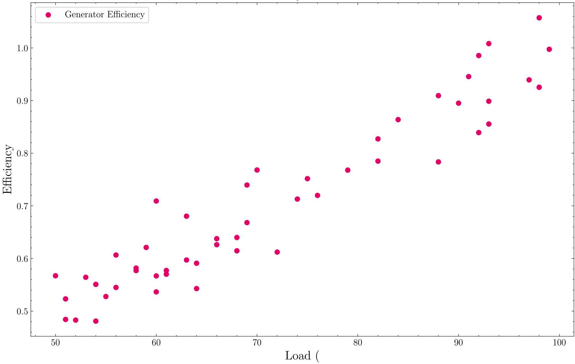
Efficiency vs. Load
