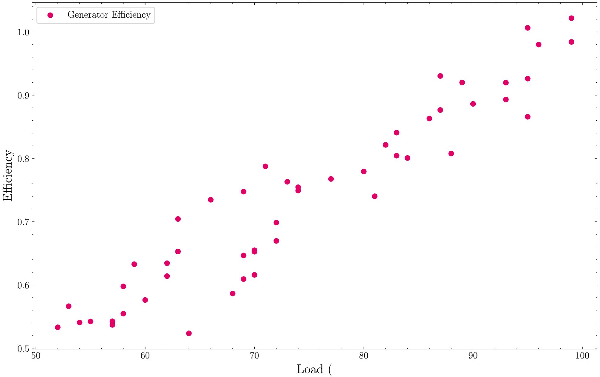
Efficiency vs. Load
