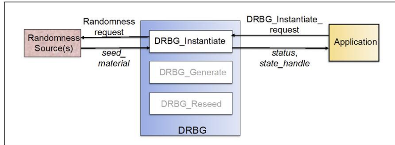
Fig. 5. DRBG_Instantiate request
