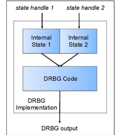
Fig. 1. DRBG instantiations
