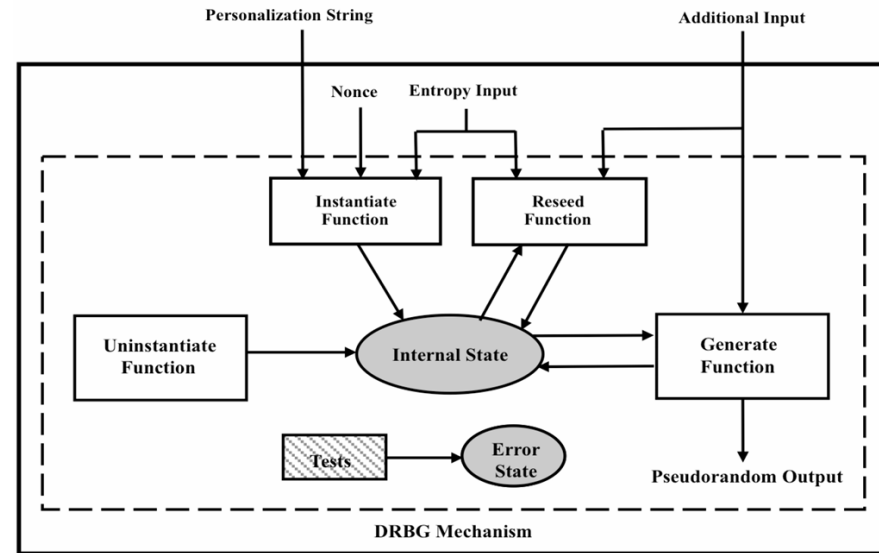
Figure 1: DRBG Functional Model
