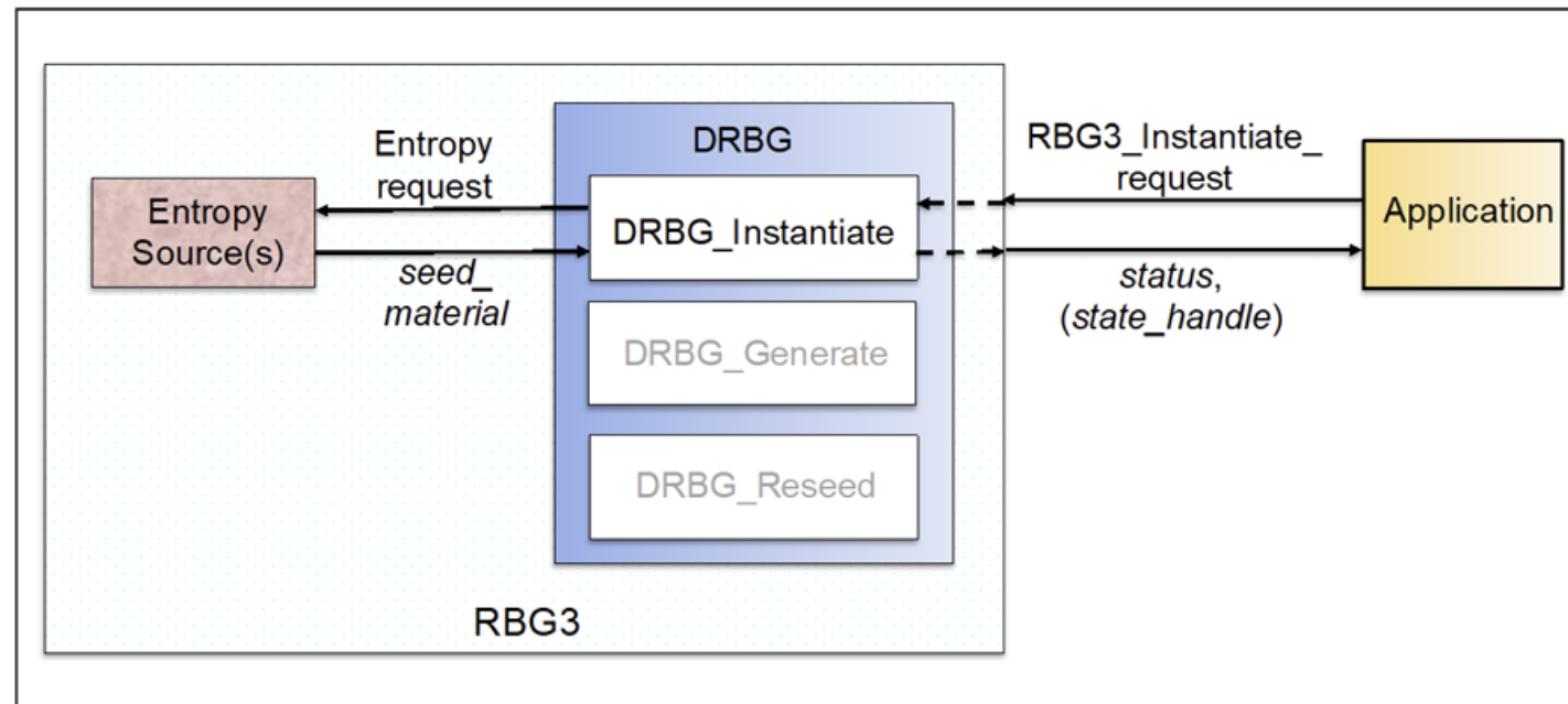
Fig. 12. RBG3(XOR) or RBG3(RS) instantiation request
