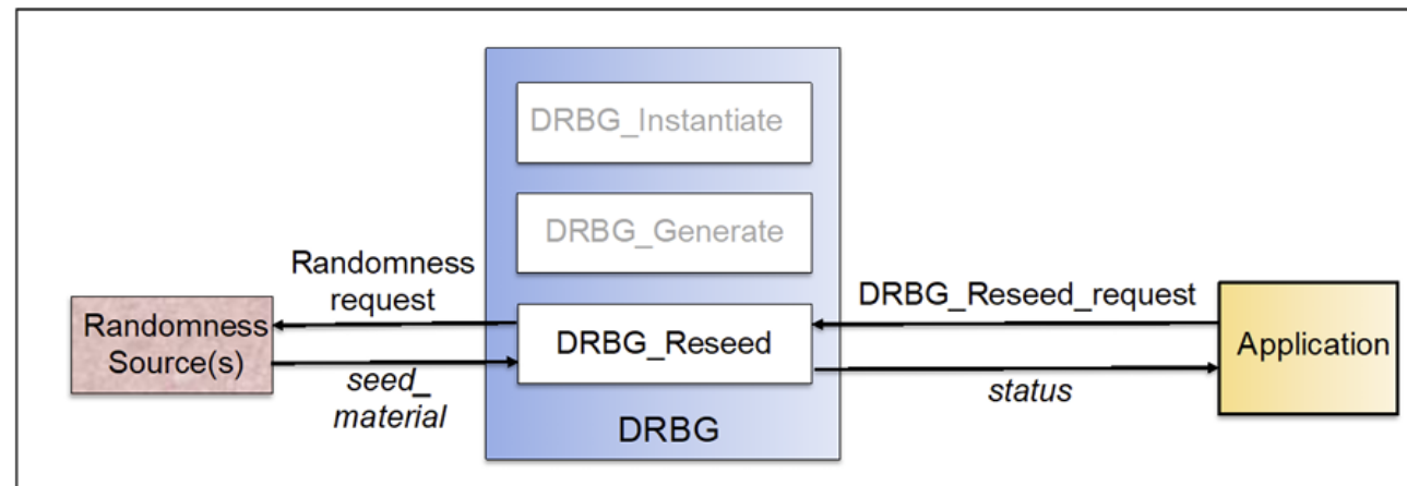
Fig. 9. DRBG_Reseed_request
