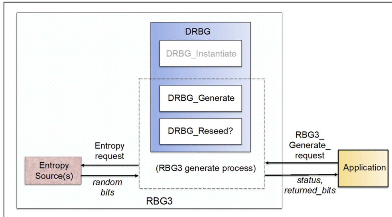
Fig. 14. Generic RBG3 generation process
