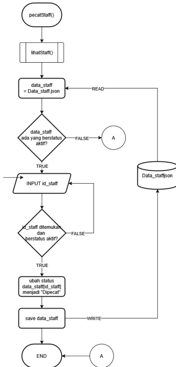
Gambar 3.7 Flowchart Pecat Staff
