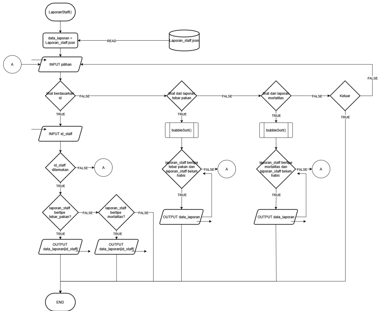
Gambar 3.15 Flowchart Laporan Staff
