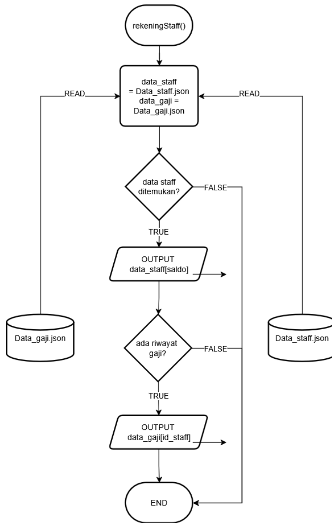
Gambar 3.23 Flowchart Rekening Staff
