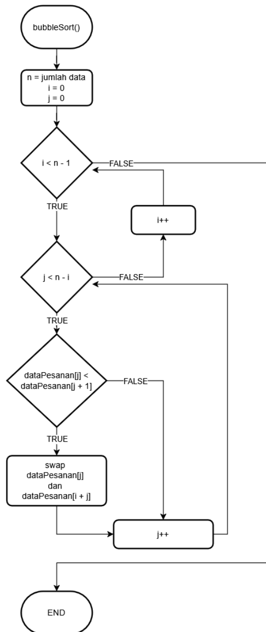
Gambar 3.24 Flowchart Bubble Sort
