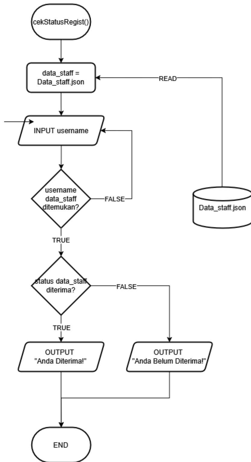
Gambar 3.20 Flowchart Cek Status Regist
