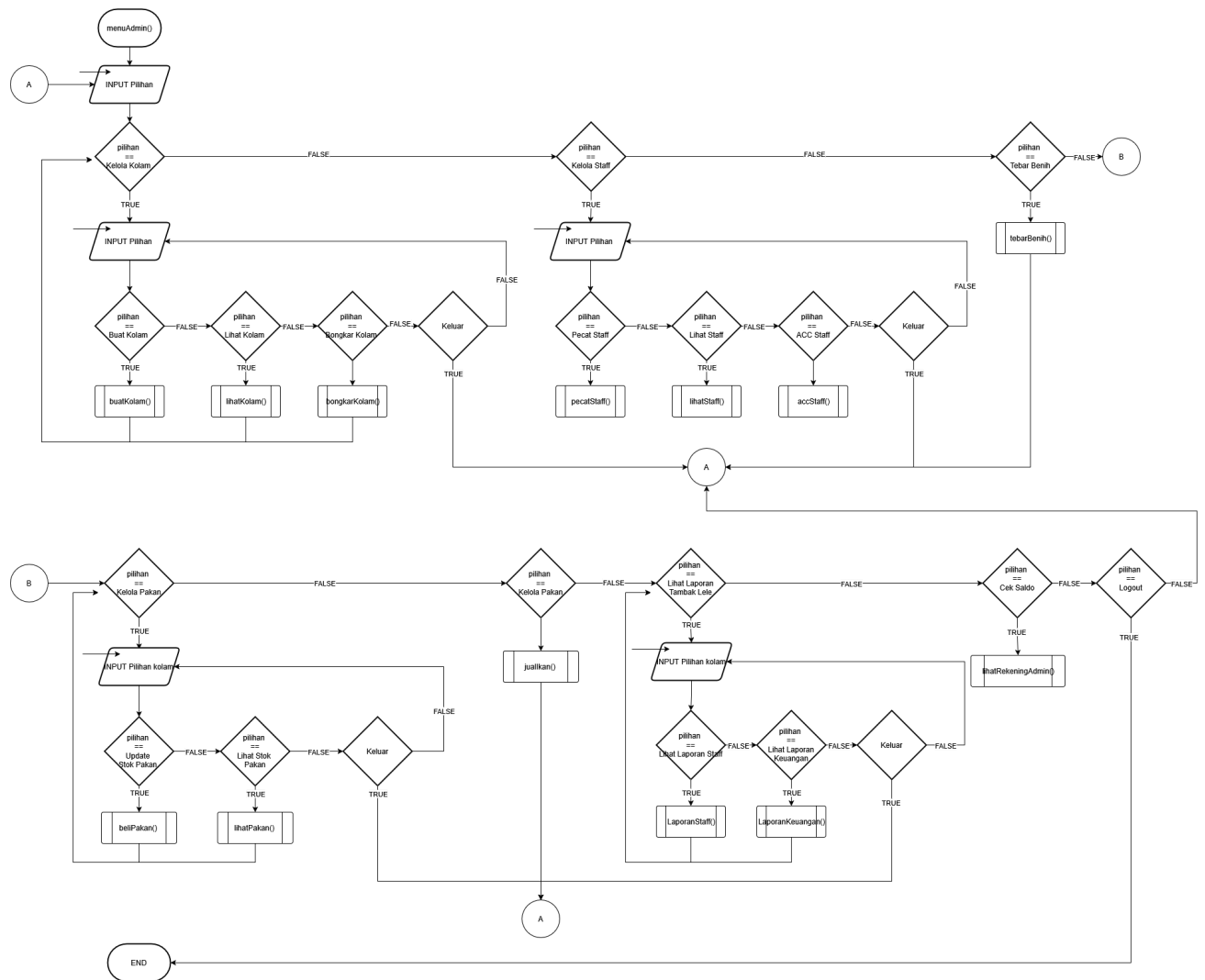
Gambar 3.2 Flowchart Menu Admin
