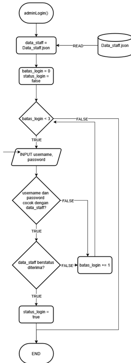
Gambar 3.19 Flowchart Login Staff
