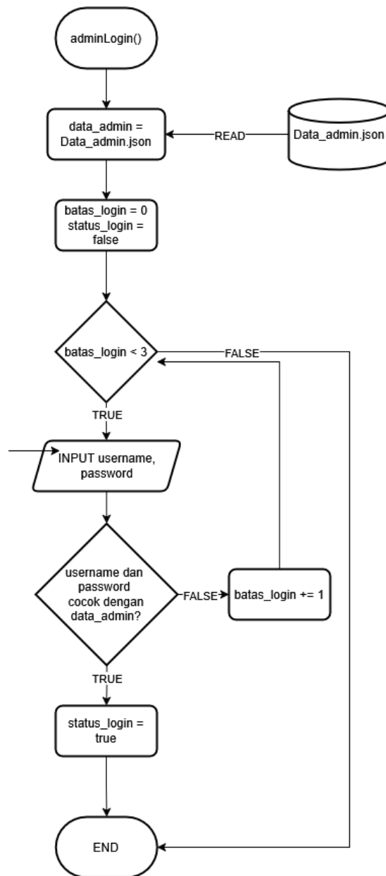
Gambar 3.3 Flowchart Login Admin
