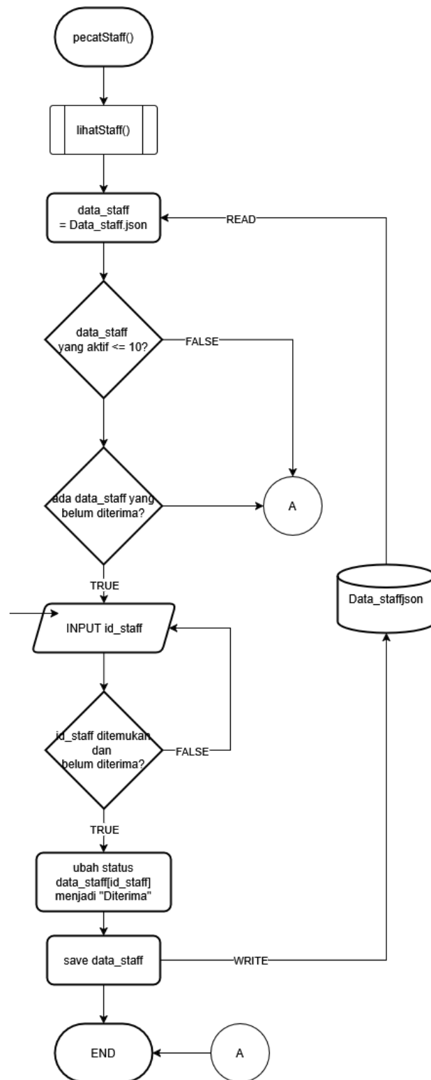
Gambar 3.8 Flowchart Acc Staff
