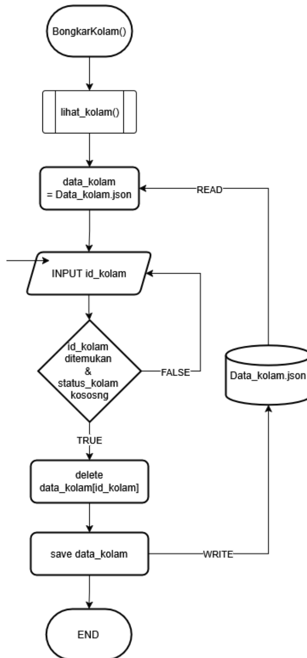
Gambar 3.5 Flowchart Bongkar Kolam
