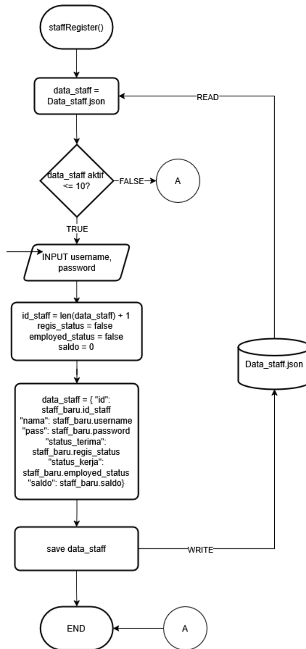
Gambar 3.18 Flowchart Regist Staff
