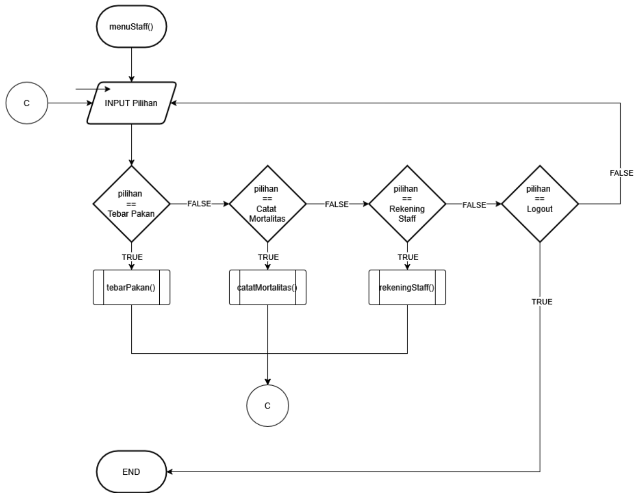
Gambar 3.17 Flowchart Menu Staff
