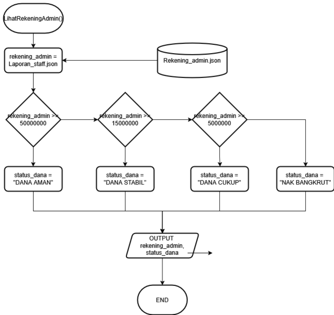
Gambar 3.16 Flowchart Rekening Admin
