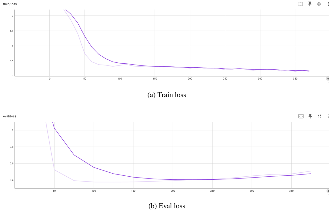
Figure 4.1. Label-only losses: rapid early train loss compression; eval loss reaches minimum near 180–220 steps then rises.
