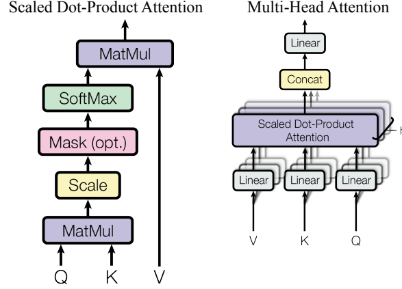
Figure 2: (left) Scaled Dot-Product Attention. (right) Multi-Head Attention consists of several attention layers running in parallel.
