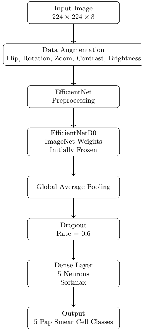
Figure 1: Architecture of the Pap Smear Cell Classification Model Based on EfficientNetB0
