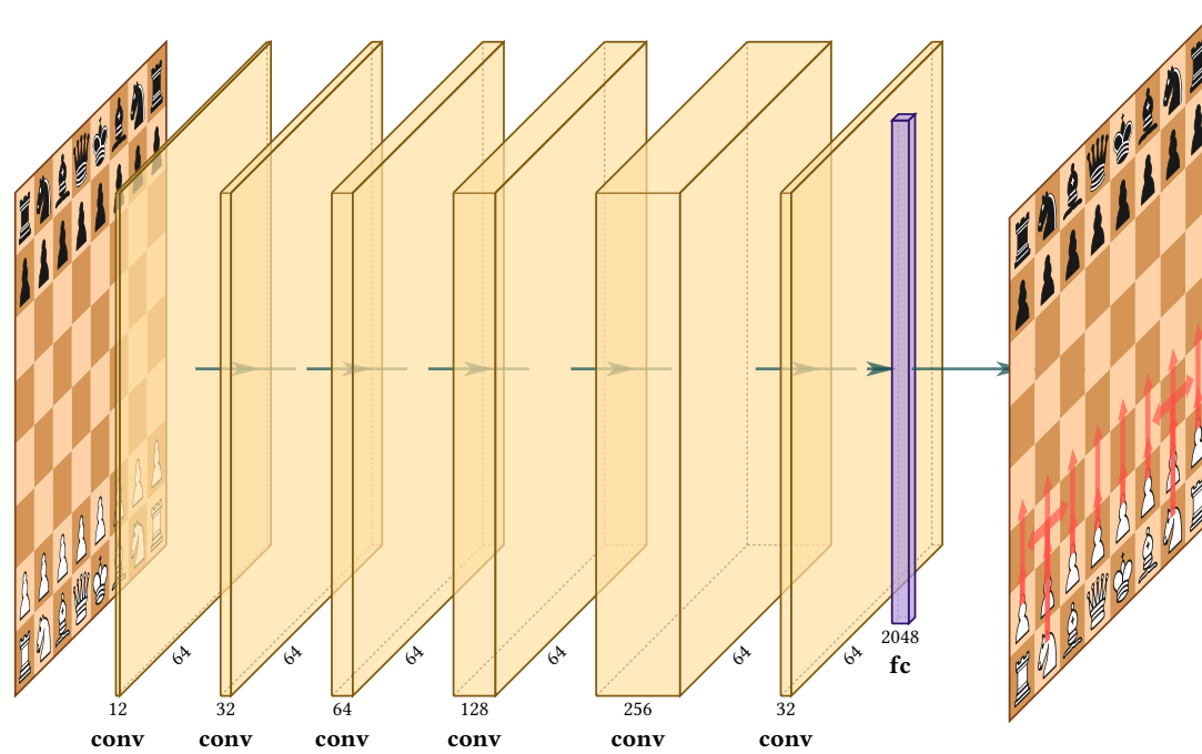
Figure 1: convolutional model
