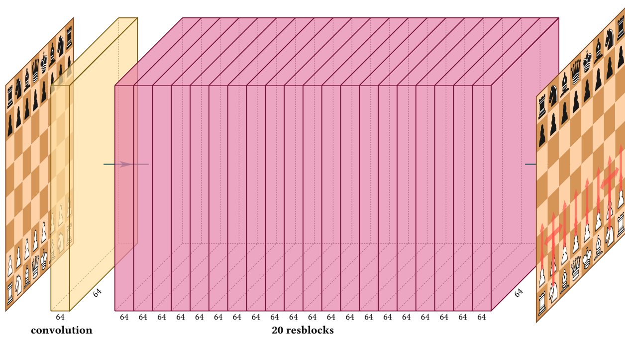
Figure 1: residual block model
