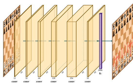
Figure 1: Architecture of the convolutional model used.
