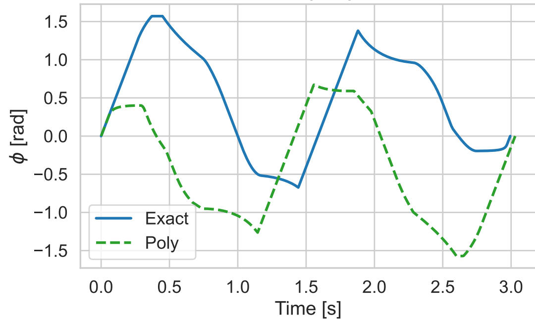
Steering Angle
