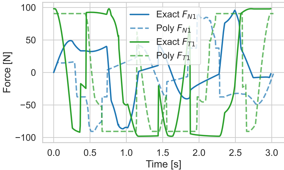
Front Axle Forces
