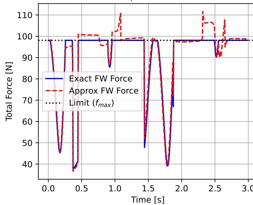
FW Slip Constraints
