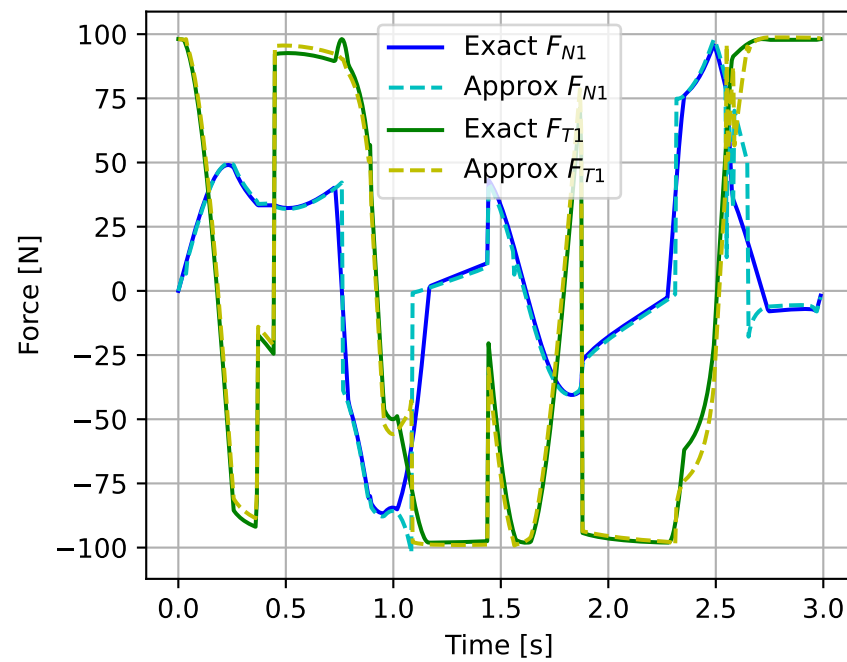
Front Forces vs Time
