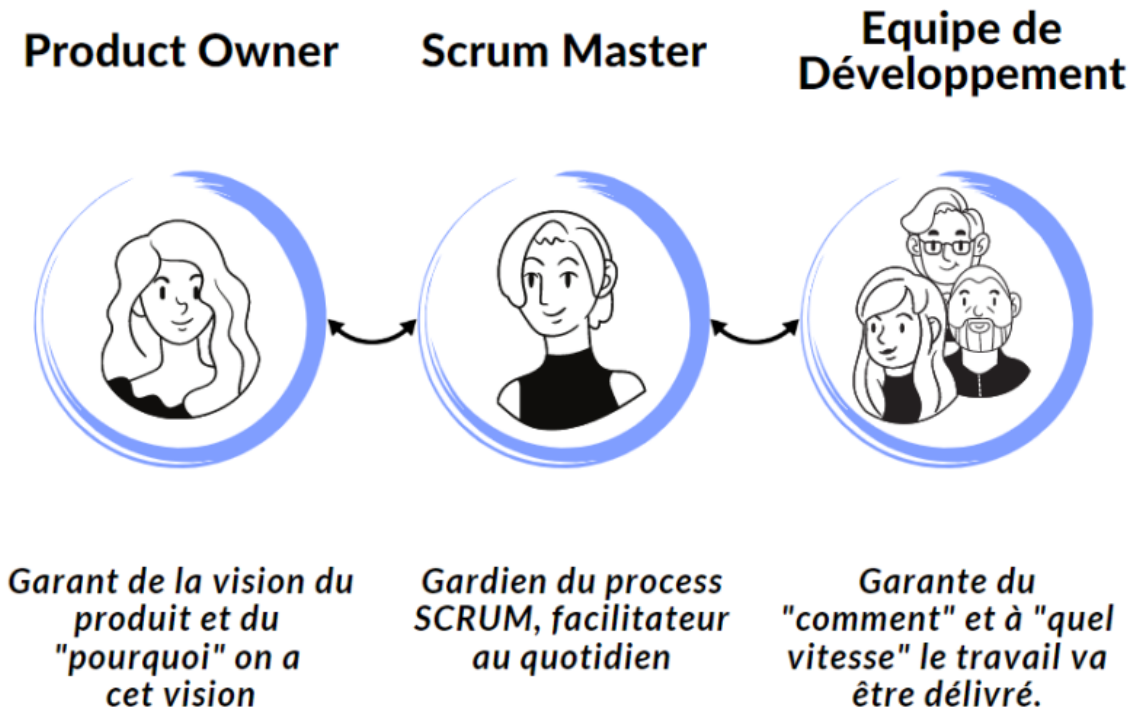
FIGURE 2.2 – Rôles Scrum.
