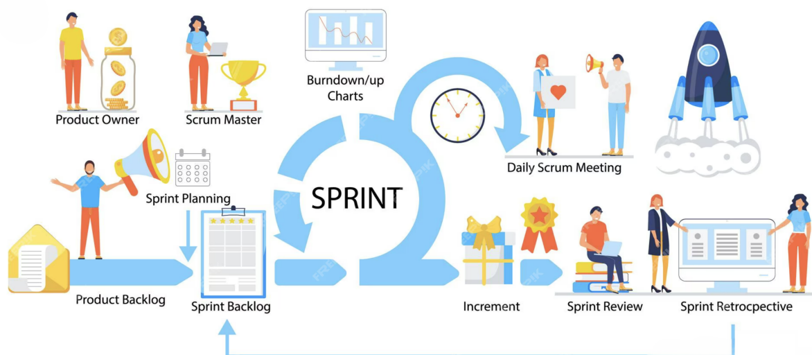
FIGURE 2.1 – Processus Scrum.
