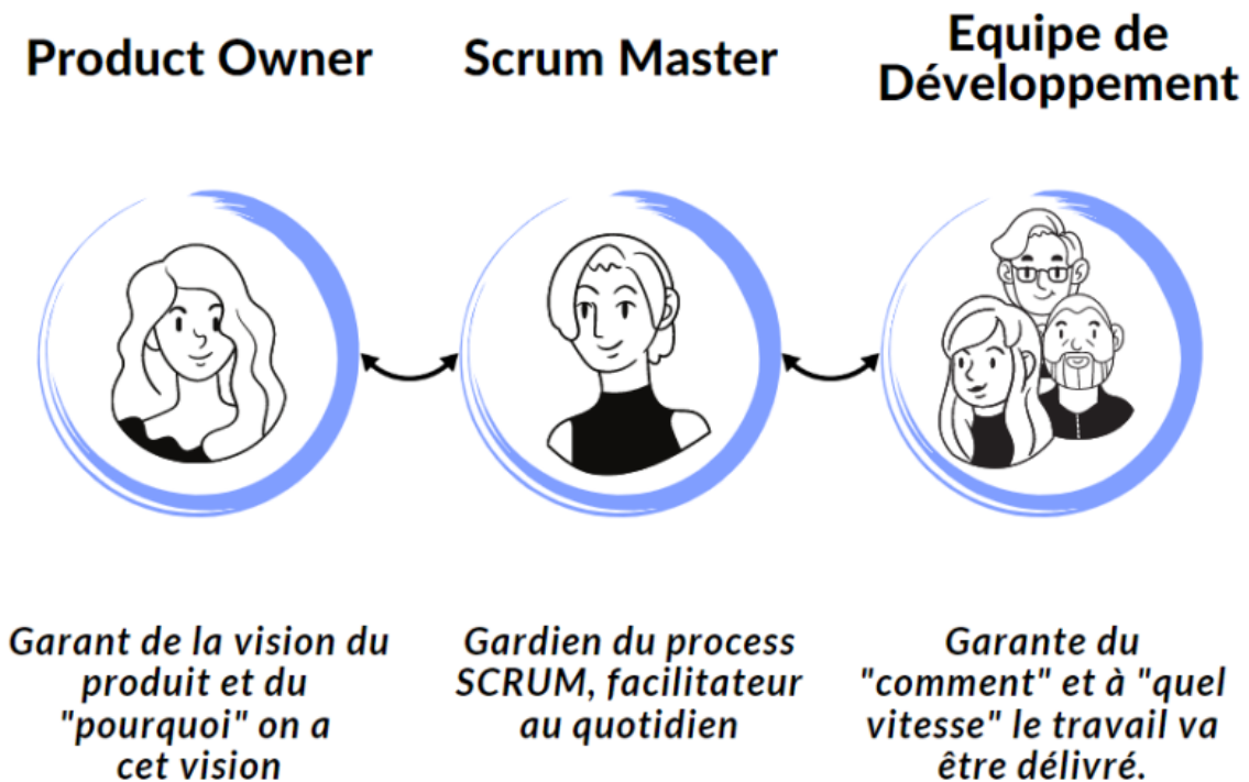
FIGURE 2.2 – Rôles Scrum.
