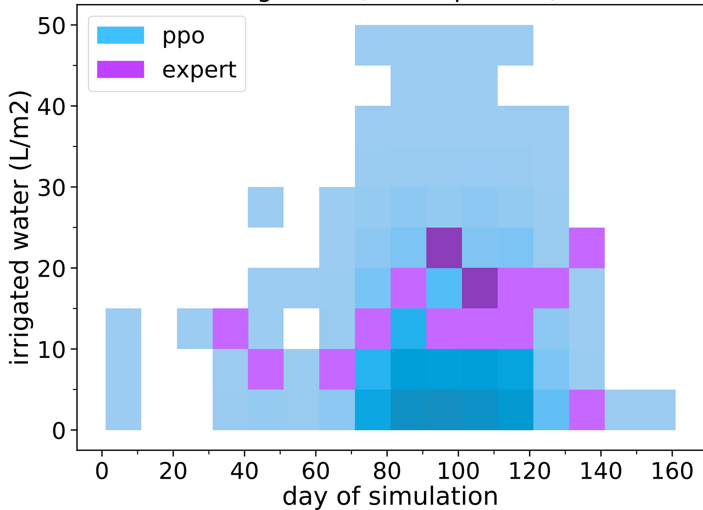
Irrigations (1000 episodes)
