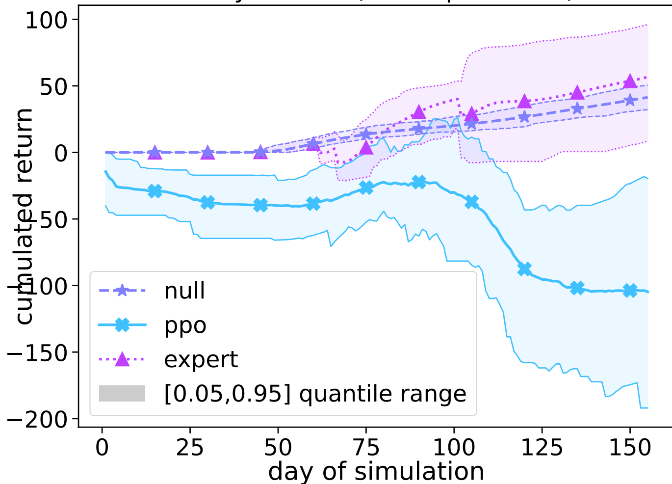
Policy returns (100 replications)
