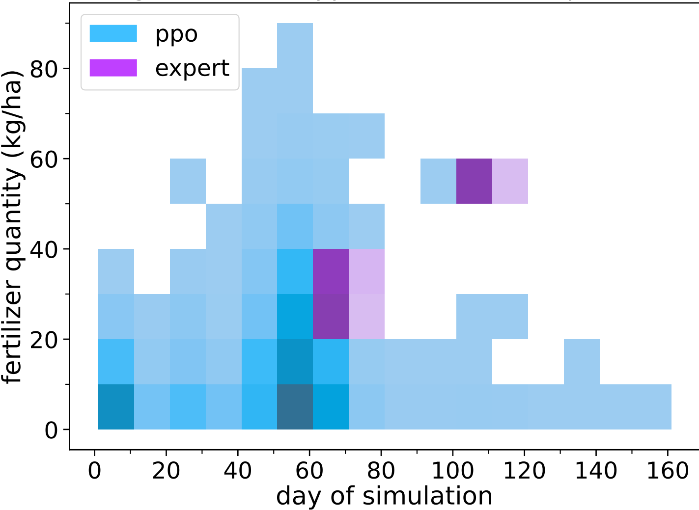
Nitrogen fertilizer applications (1000 replications)
