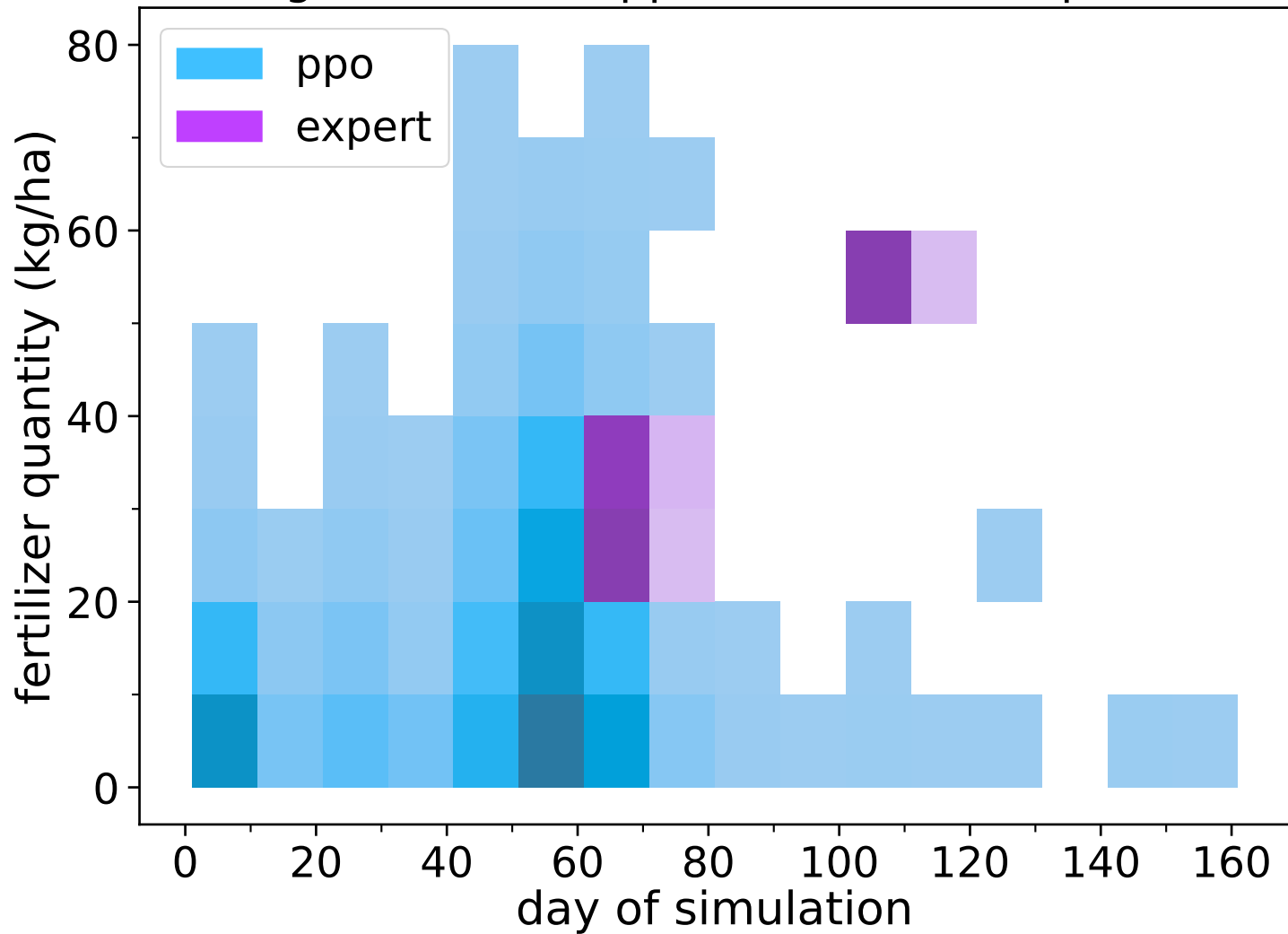
Nitrogen fertilizer applications (1000 episodes)
