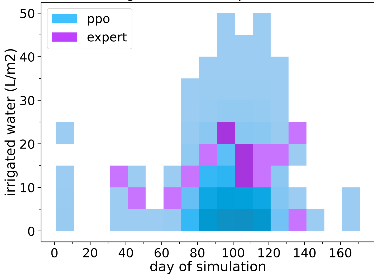
Irrigations (1000 replications)
