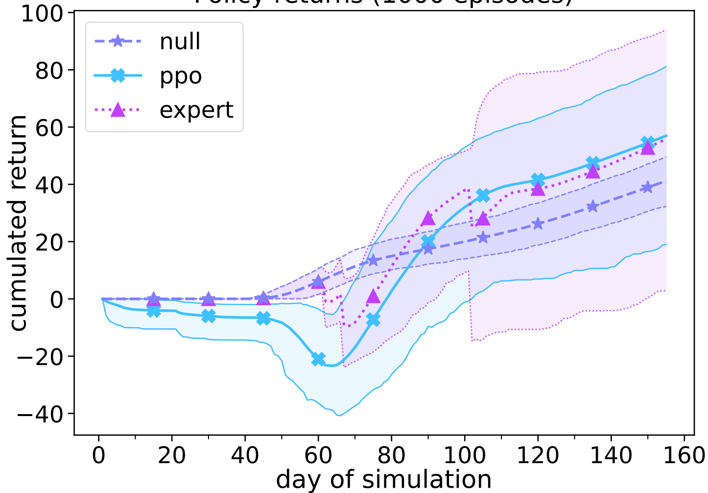
Policy returns (1000 episodes)
