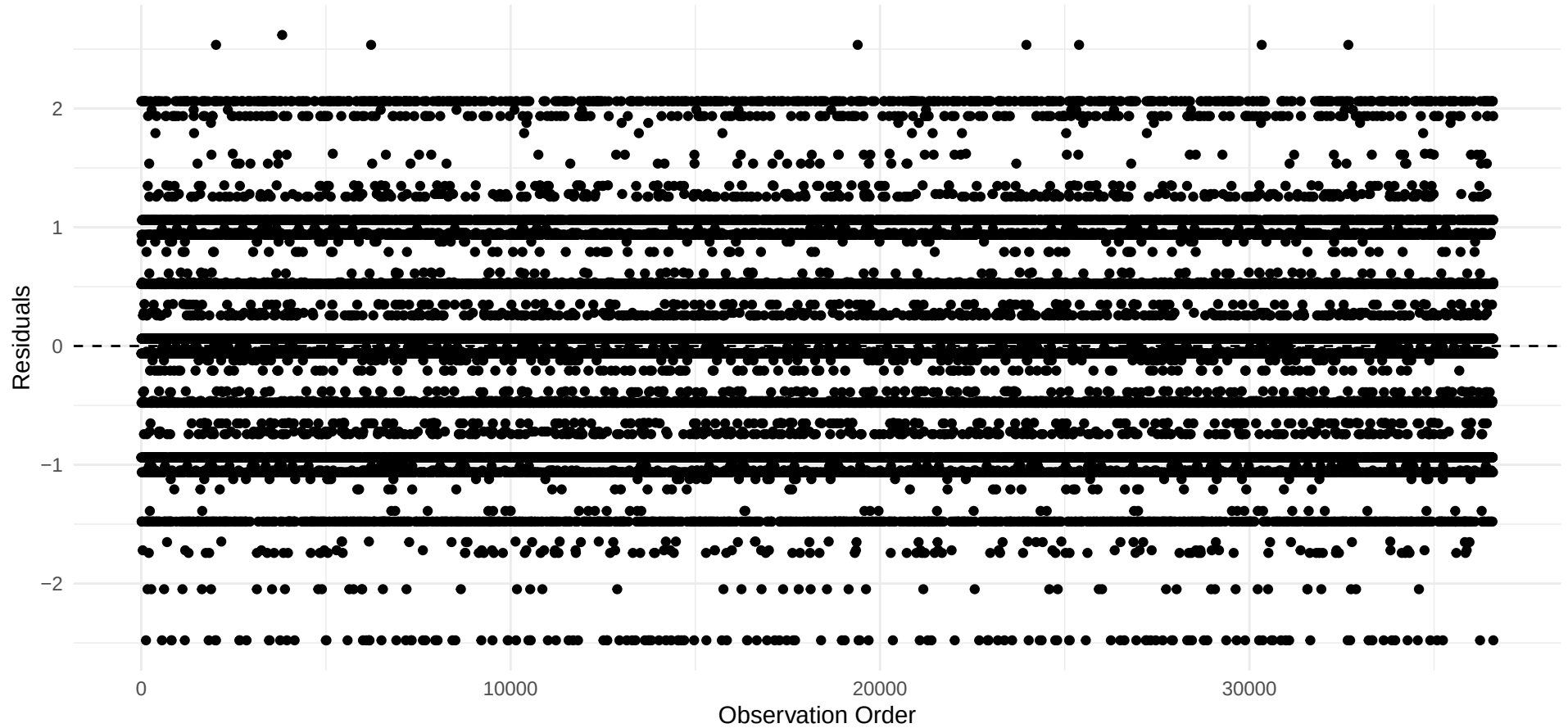
Residuals vs Observation Order (Independence Check)
