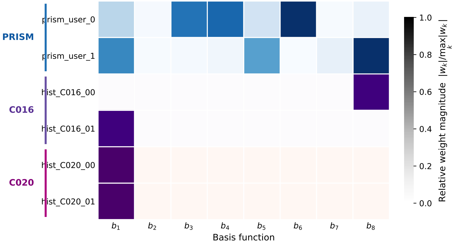
User weight vectors over LoRe basis
