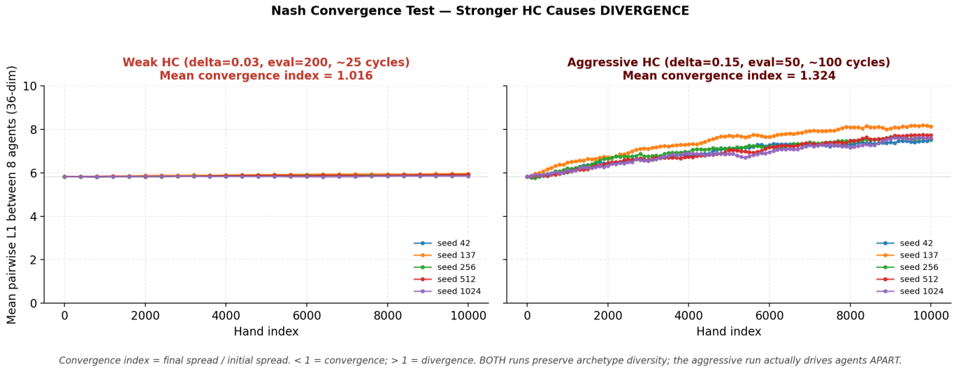
Fig. S4. The 8-agent population becomes dispersed in parameter space. Averaged pairwise L_1 distance between all eight agents in a 36-dimensional parameter space over 10,000 hands of unbounded hill-climbing. (Left) With weak HC ( \delta = 0.03 ), agents barely move. (Right) Aggressive HC ( \delta = 0.15 ) spreads the population out on every seed. A ratio of final-to-initial cluster spread > 1 implies the agents become more dispersed at end-of-run than at the start.
