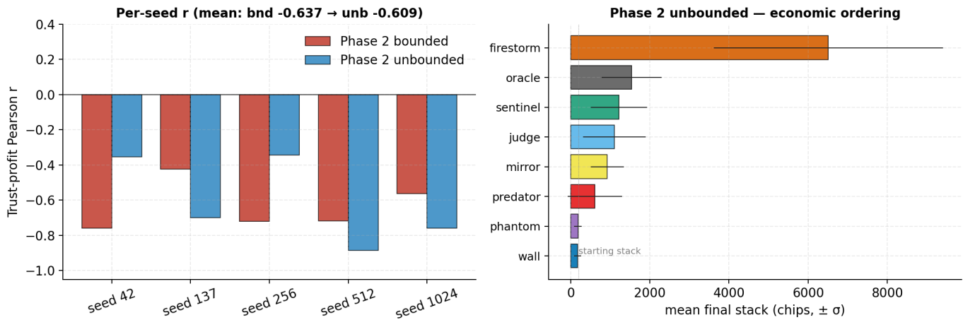
Fig. S3. Bounded versus unbounded hill-climbing per seed. The left of each pair of bars is r_{tp} for bounded Phase 2 hill-climbing; the right is r_{tp} for aggressive Phase 2* hill-climbing, for each of the five canonical seeds. When the bounding constraints are relaxed and the optimiser's step size is increased fivefold, r_{tp} increases by only +0.028 on average, and across seeds the variance in r_{tp} nearly triples.
