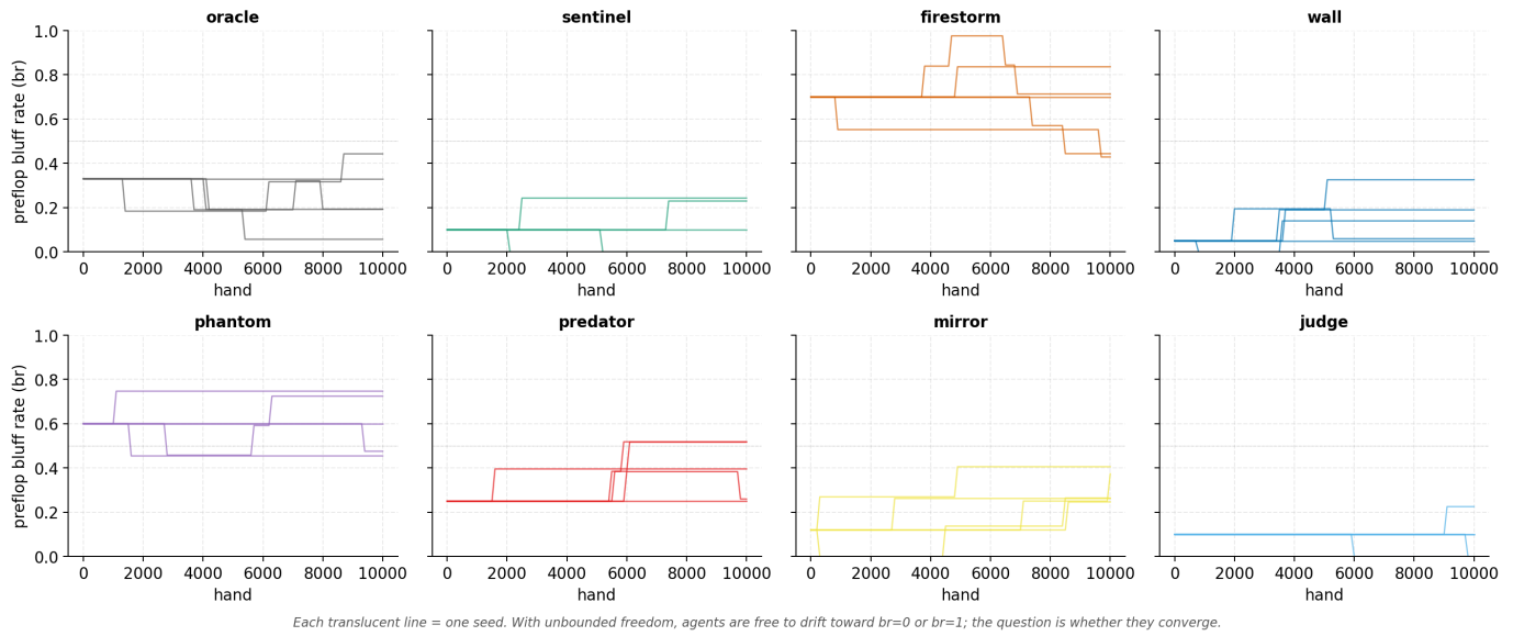
Fig. S2. Per-archetype preflop bluff-rate drift under aggressive unbounded hill-climbing. Each panel is one archetype and each translucent line is one of the five seeds. Every archetype's bluff rate wanders substantially over the run, yet the panels do not converge on a common profile (the corresponding mean L_1 parameter drift is 3.4).
