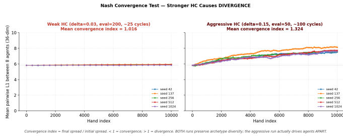
Figure 3. The 8-agent population becomes dispersed in parameter space. Averaged pairwise L_1 distance between all eight agents in a 36-dimensional parameter space over 10,000 hands of unbounded hill-climbing. (Left) With weak HC ( \delta = 0.03 ), agents barely move. (Right) Aggressive HC ( \delta = 0.15 ) spreads the population out on every seed. A ratio of final-to-initial cluster spread > 1 implies the agents become more dispersed at end-of-run than at the start.
