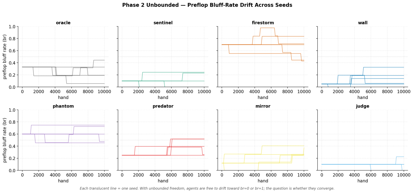
Figure 4. Per-archetype preflop bluff-rate drift under aggressive unbounded hill-climbing. Each panel is one archetype and each translucent line is one of the five seeds. Every archetype’s bluff rate wanders substantially over the run, yet the panels do not converge on a common profile (the corresponding mean L_1 parameter drift is 3.4).
