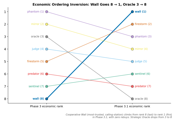
Figure 5. Economic ordering inverts from Phase 3 to Phase 3.1. Wall (trust \approx 0.85 , highest of any archetype) was rank 8 of 8 in Phase 3 with \sim 9 rebuys per seed and becomes rank 1 of 8 in Phase 3.1 with zero rebuys. Firestorm climbs from rank 5 in Phase 3 to rank 2 in Phase 3.1.
