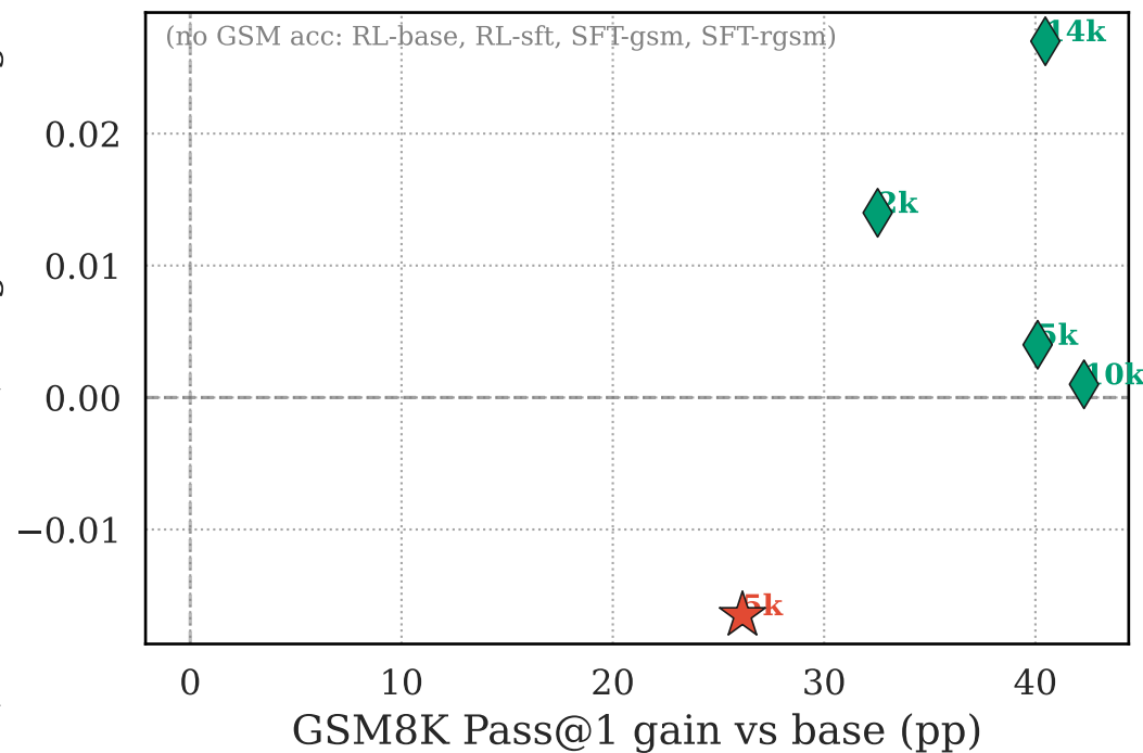
SQuAD-Completion BPB
