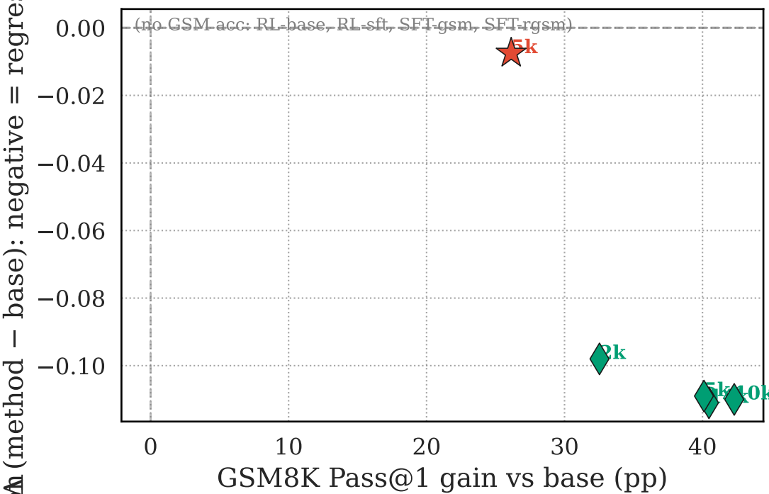
OpenBookQA
